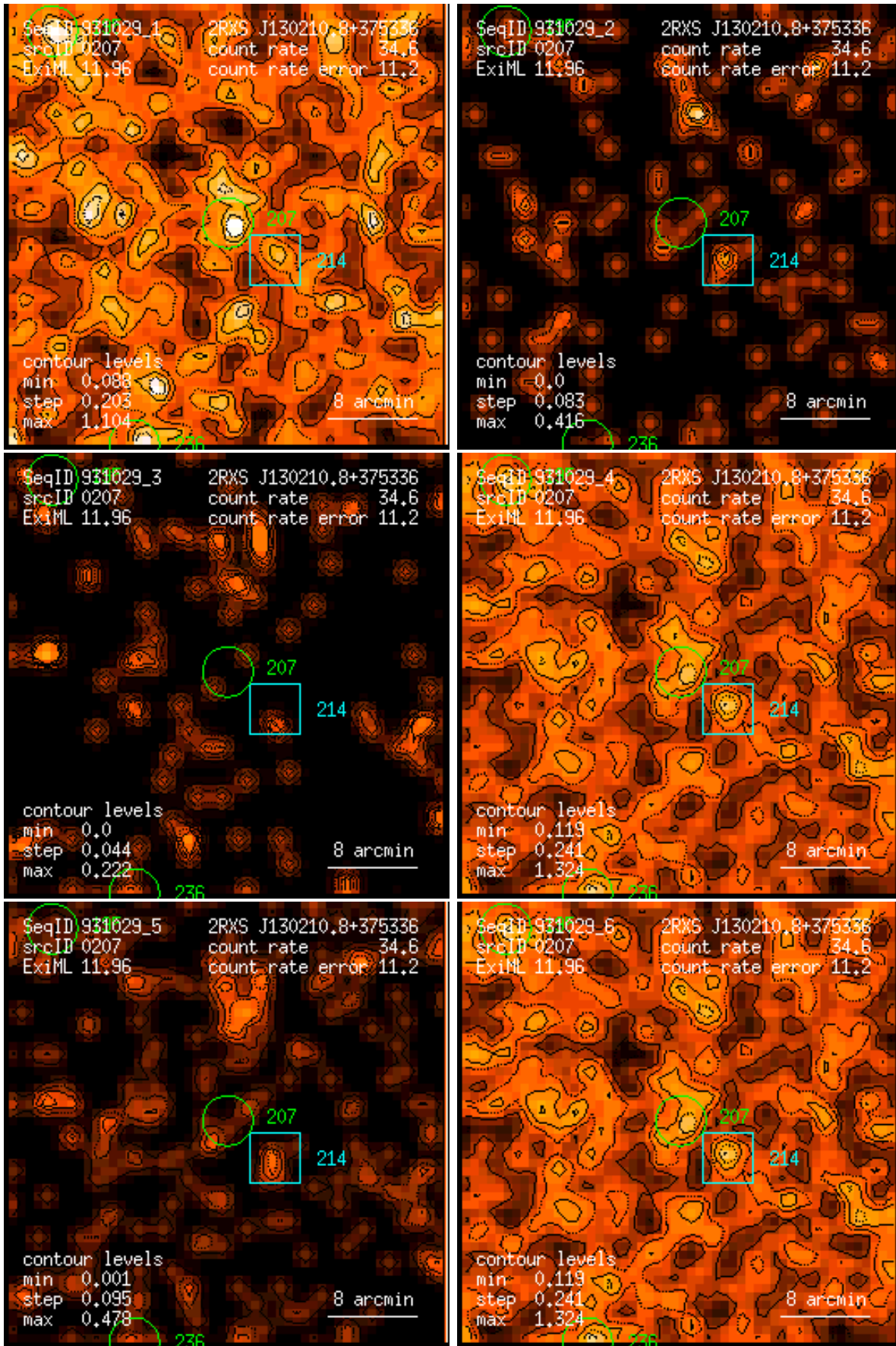
Figure 207: RASS 931029: detection 0207: band rate images, Gaussian filter: (1) PSPC channels 11 – 41, (2) 52 – 90, (3) 91 – 201, (4) 11 – 235, (5) 52 – 201, (6) 11 – 201. Broad band rates in counts/ks. Band rate contour levels in counts/ks/arcmin 2 .
