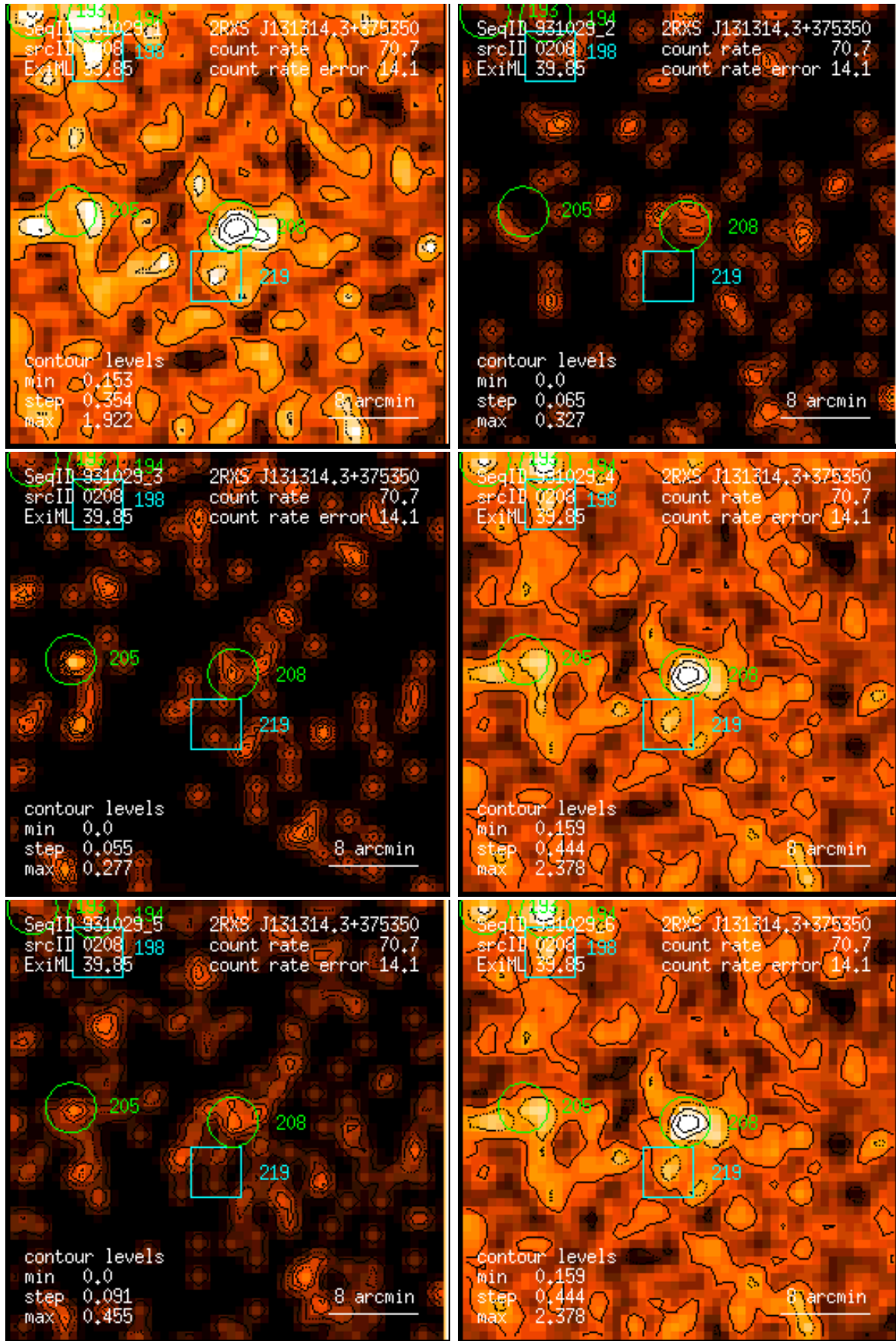
Figure 208: RASS 931029: detection 0208: band rate images, Gaussian filter: (1) PSPC channels 11 – 41, (2) 52 – 90, (3) 91 – 201, (4) 11 – 235, (5) 52 – 201, (6) 11 – 201. Broad band rates in counts/ks. Band rate contour levels in counts/ks/arcmin 2 .
