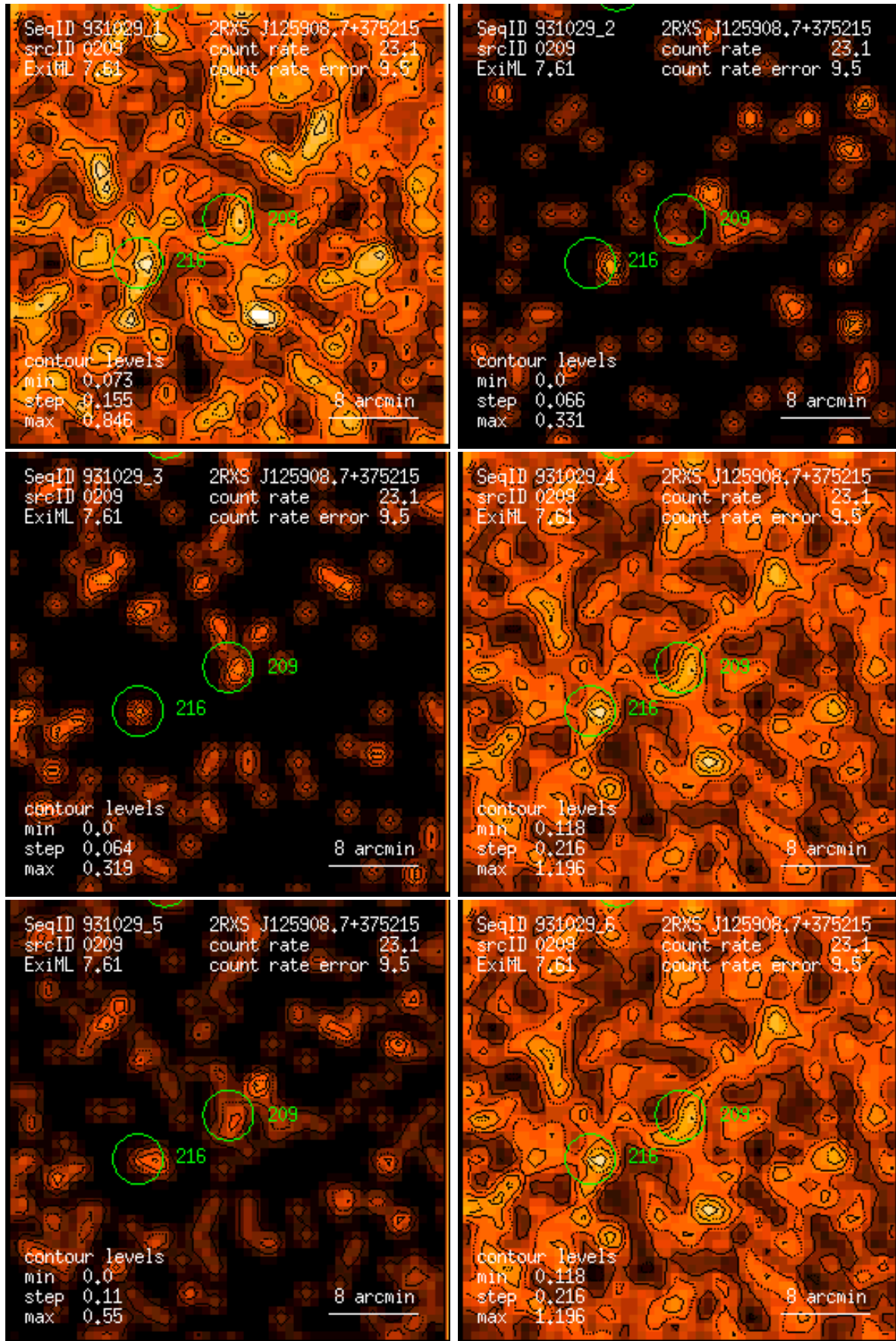
Figure 209: RASS 931029: detection 0209: band rate images, Gaussian filter: (1) PSPC channels 11 – 41, (2) 52 – 90, (3) 91 – 201, (4) 11 – 235, (5) 52 – 201, (6) 11 – 201. Broad band rates in counts/ks. Band rate contour levels in counts/ks/arcmin 2 .
