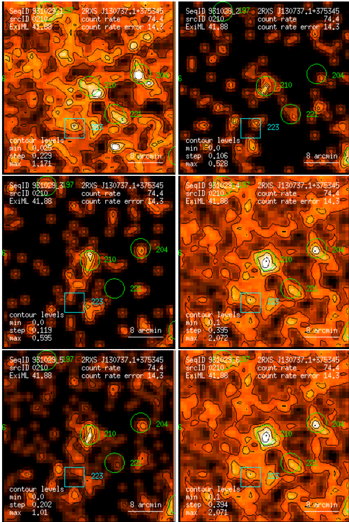
Figure 210: RASS 931029: detection 0210: band rate images, Gaussian filter: (1) PSPC channels 11 – 41, (2) 52 – 90, (3) 91 – 201, (4) 11 – 235, (5) 52 – 201, (6) 11 – 201. Broad band rates in counts/ks. Band rate contour levels in counts/ks/arcmin 2 .
