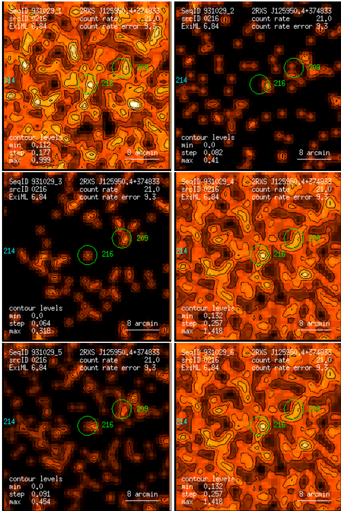
Figure 216: RASS 931029: detection 0216: band rate images, Gaussian filter: (1) PSPC channels 11 – 41, (2) 52 – 90, (3) 91 – 201, (4) 11 – 235, (5) 52 – 201, (6) 11 – 201. Broad band rates in counts/ks. Band rate contour levels in counts/ks/arcmin 2 .
