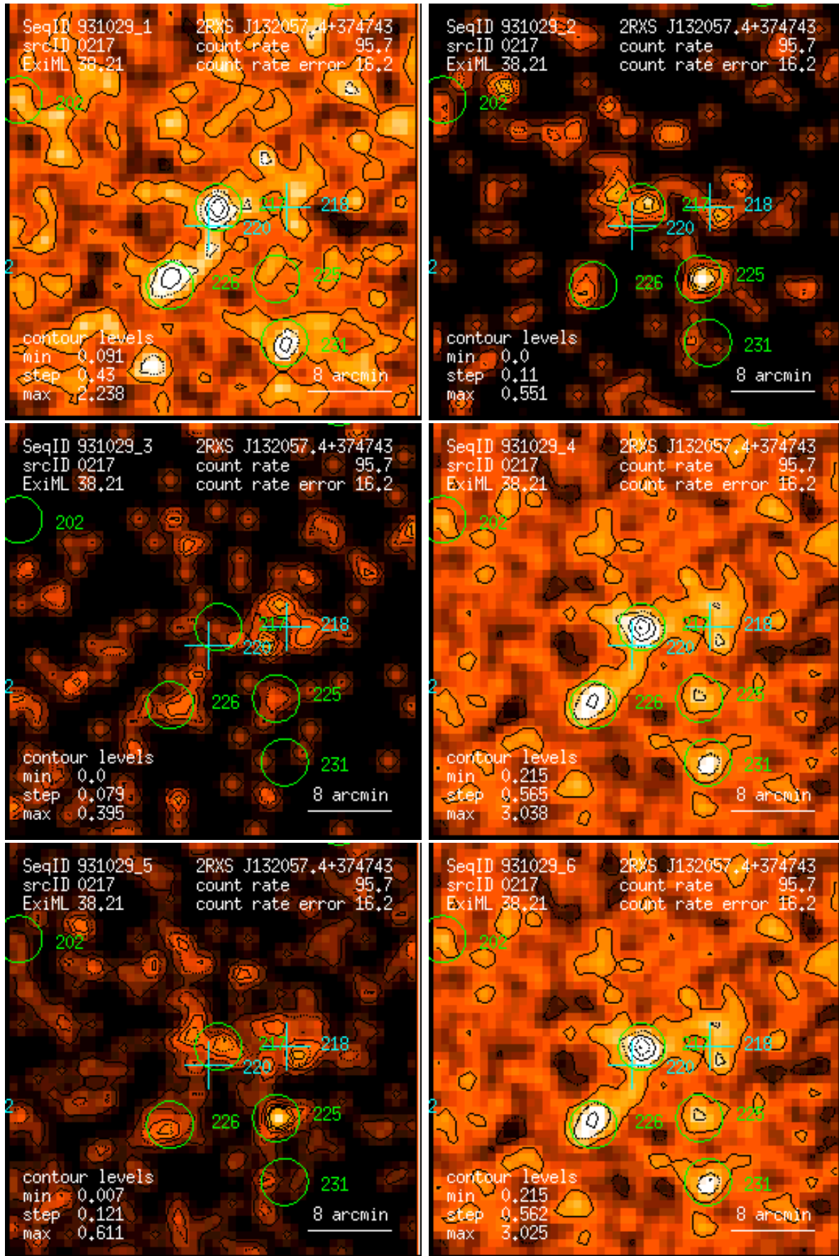
Figure 217: RASS 931029: detection 0217: band rate images, Gaussian filter: (1) PSPC channels 11 – 41, (2) 52 – 90, (3) 91 – 201, (4) 11 – 235, (5) 52 – 201, (6) 11 – 201. Broad band rates in counts/ks. Band rate contour levels in counts/ks/arcmin 2 .
