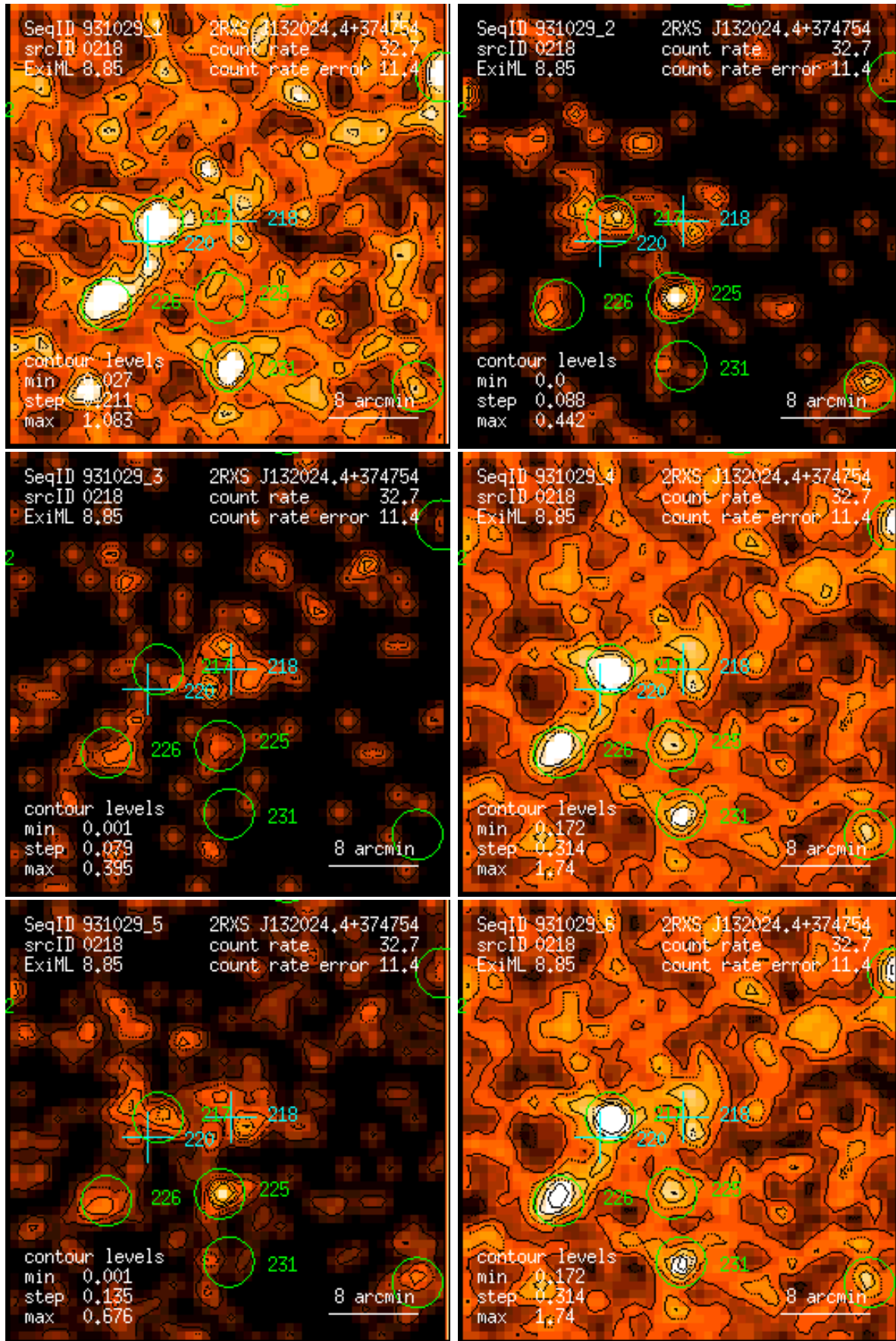
Figure 218: RASS 931029: detection 0218: band rate images, Gaussian filter: (1) PSPC channels 11 – 41, (2) 52 – 90, (3) 91 – 201, (4) 11 – 235, (5) 52 – 201, (6) 11 – 201. Broad band rates in counts/ks. Band rate contour levels in counts/ks/arcmin 2 .
