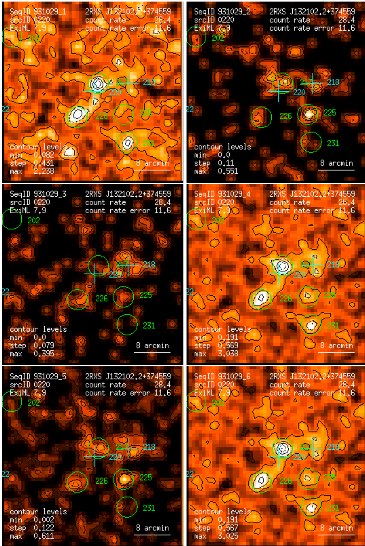
Figure 220: RASS 931029: detection 0220: band rate images, Gaussian filter: (1) PSPC channels 11 – 41, (2) 52 – 90, (3) 91 – 201, (4) 11 – 235, (5) 52 – 201, (6) 11 – 201. Broad band rates in counts/ks. Band rate contour levels in counts/ks/arcmin 2 .
