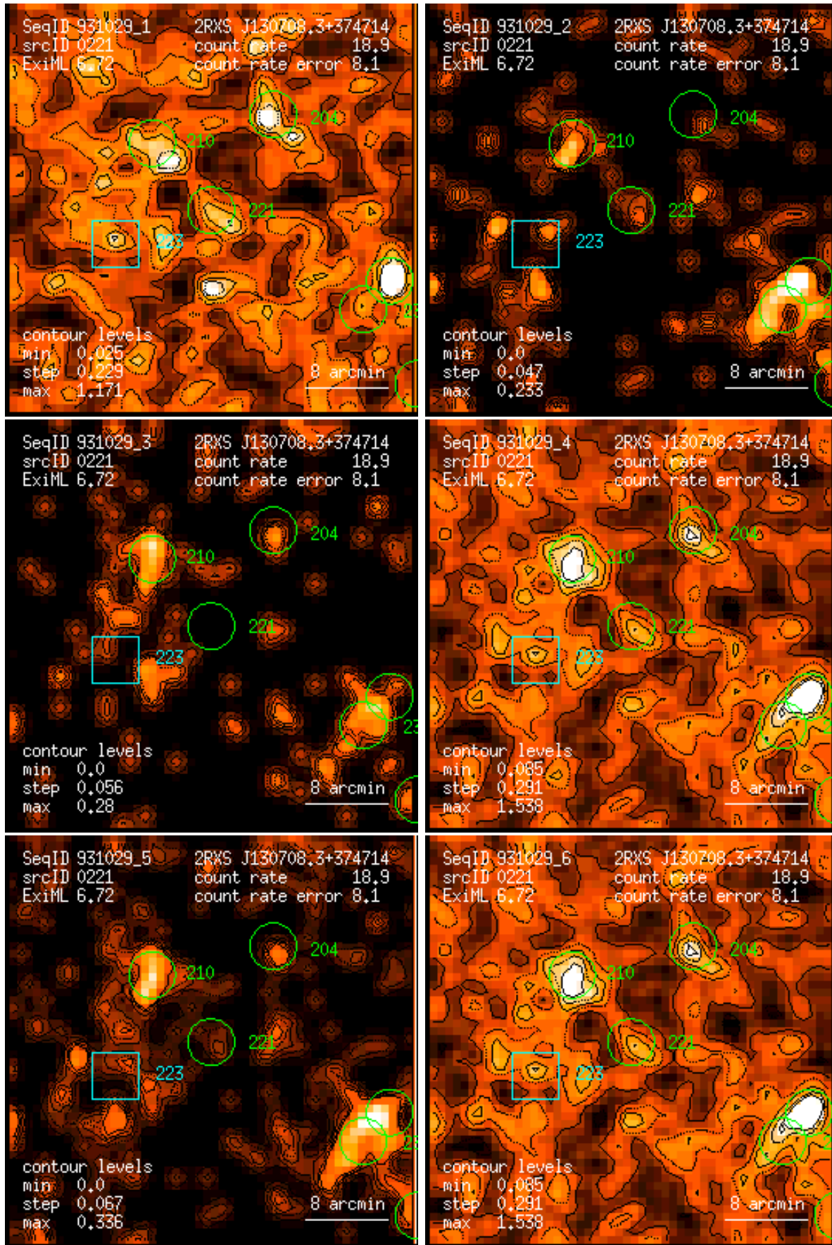
Figure 221: RASS 931029: detection 0221: band rate images, Gaussian filter: (1) PSPC channels 11 – 41, (2) 52 – 90, (3) 91 – 201, (4) 11 – 235, (5) 52 – 201, (6) 11 – 201. Broad band rates in counts/ks. Band rate contour levels in counts/ks/arcmin 2 .
