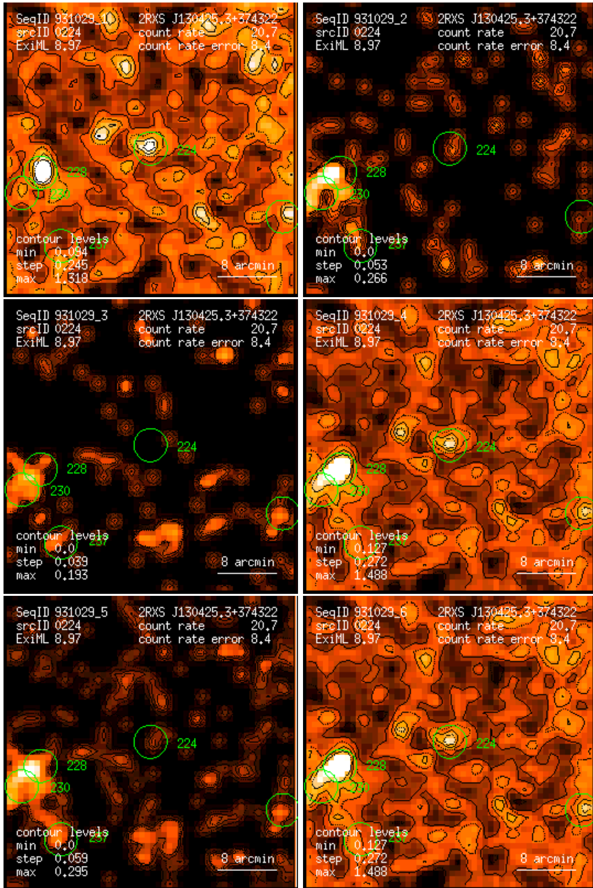
Figure 224: RASS 931029: detection 0224: band rate images, Gaussian filter: (1) PSPC channels 11 – 41, (2) 52 – 90, (3) 91 – 201, (4) 11 – 235, (5) 52 – 201, (6) 11 – 201. Broad band rates in counts/ks. Band rate contour levels in counts/ks/arcmin 2 .
