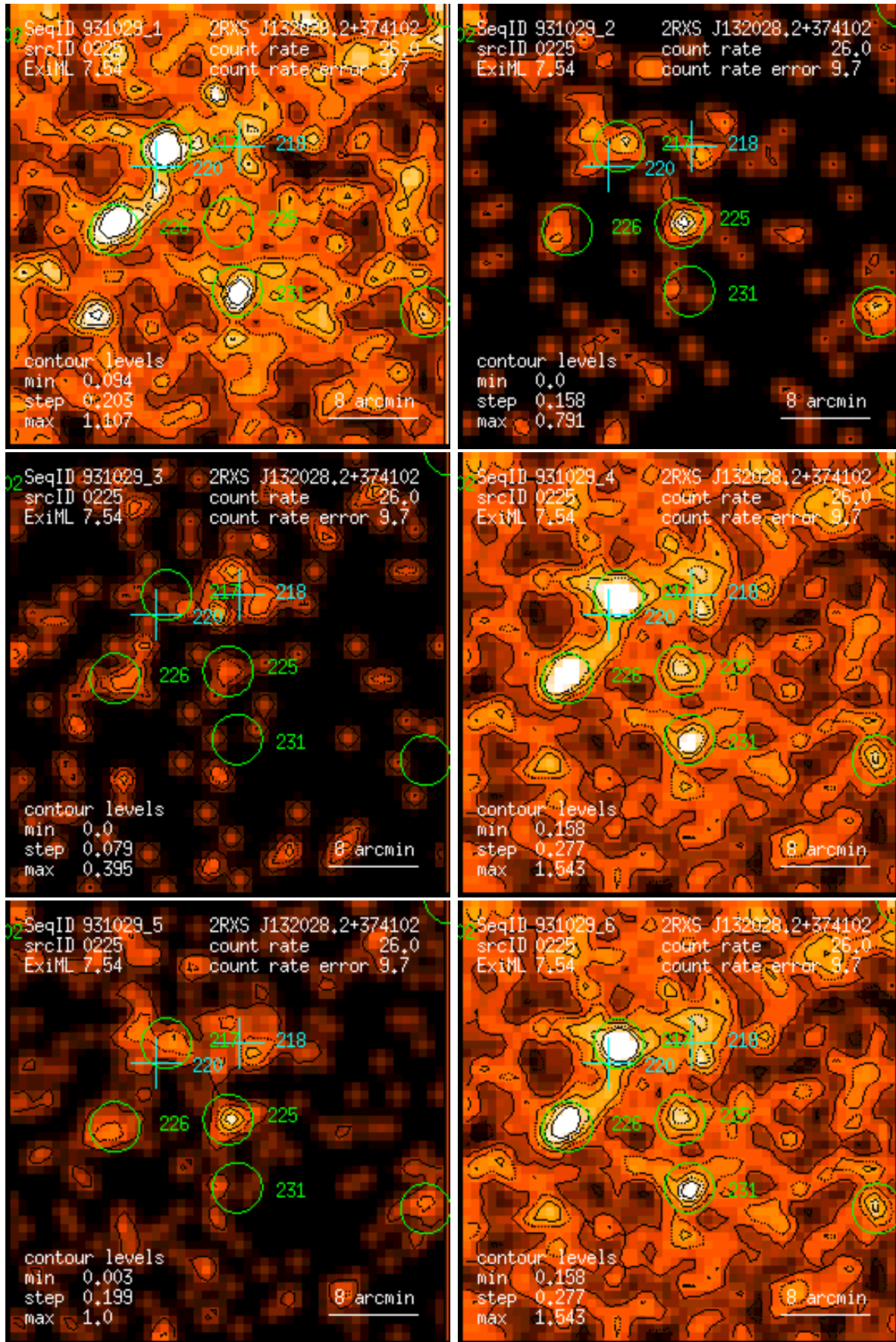
Figure 225: RASS 931029: detection 0225: band rate images, Gaussian filter: (1) PSPC channels 11 – 41, (2) 52 – 90, (3) 91 – 201, (4) 11 – 235, (5) 52 – 201, (6) 11 – 201. Broad band rates in counts/ks. Band rate contour levels in counts/ks/arcmin 2 .
