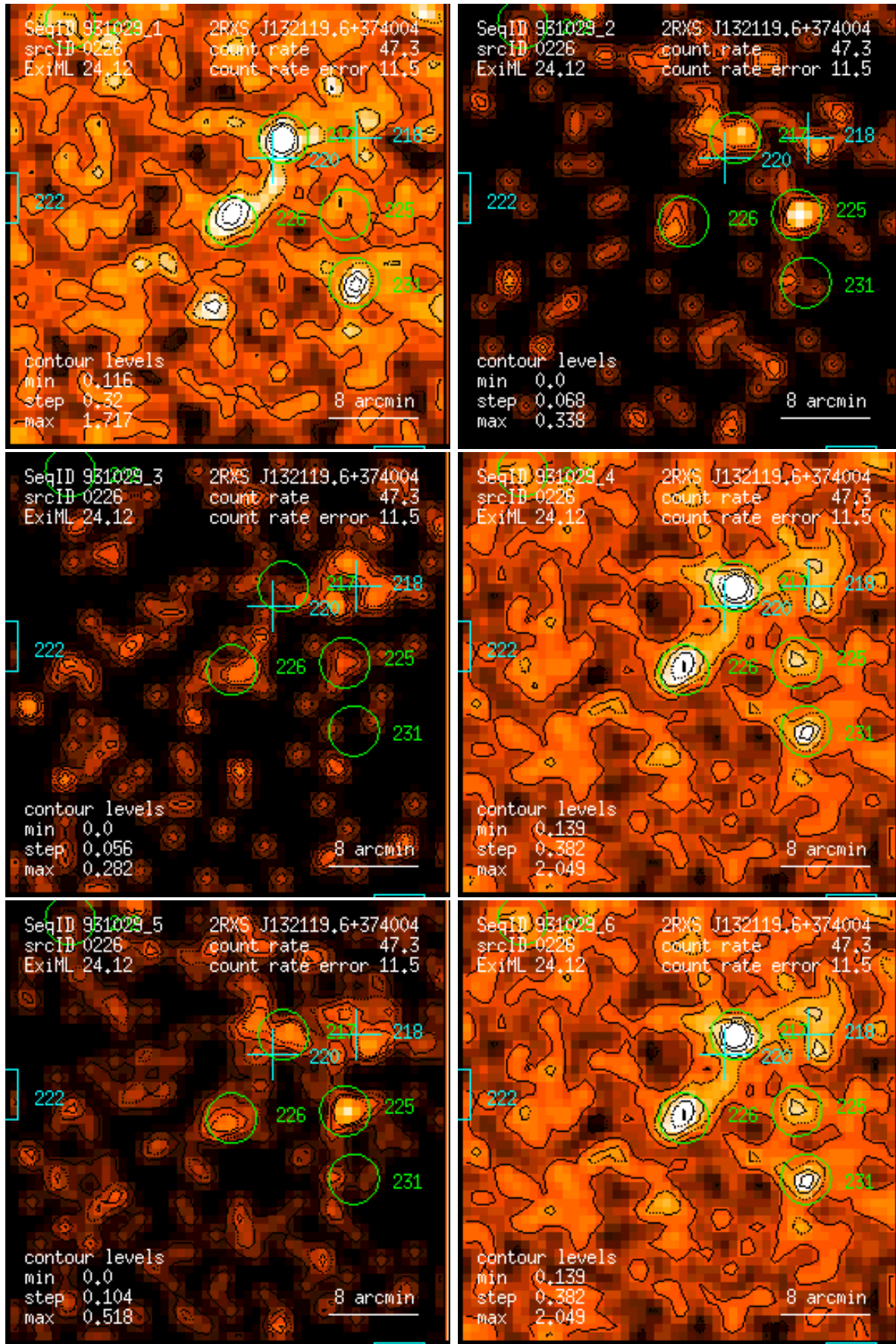
Figure 226: RASS 931029: detection 0226: band rate images, Gaussian filter: (1) PSPC channels 11 – 41, (2) 52 – 90, (3) 91 – 201, (4) 11 – 235, (5) 52 – 201, (6) 11 – 201. Broad band rates in counts/ks. Band rate contour levels in counts/ks/arcmin 2 .
