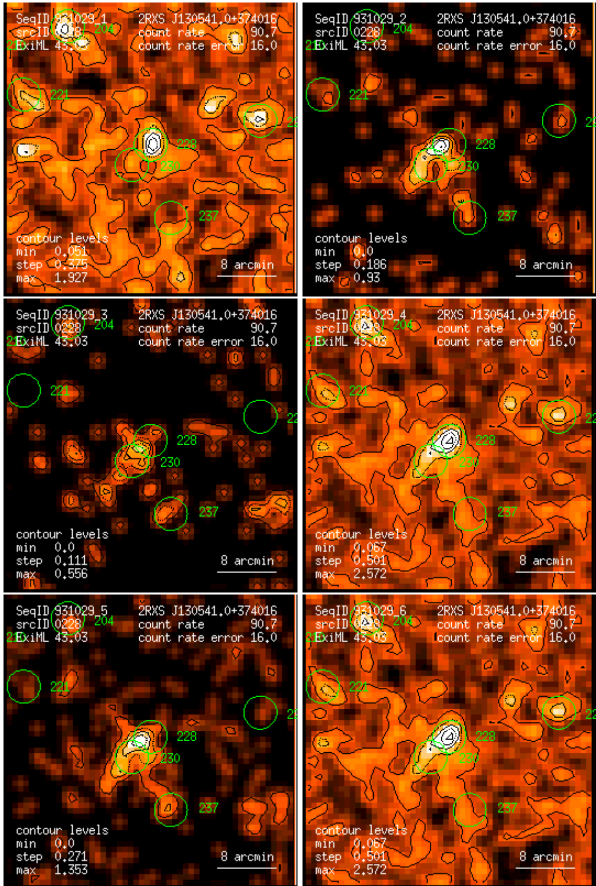
Figure 228: RASS 931029: detection 0228: band rate images, Gaussian filter: (1) PSPC channels 11 – 41, (2) 52 – 90, (3) 91 – 201, (4) 11 – 235, (5) 52 – 201, (6) 11 – 201. Broad band rates in counts/ks. Band rate contour levels in counts/ks/arcmin 2 .
