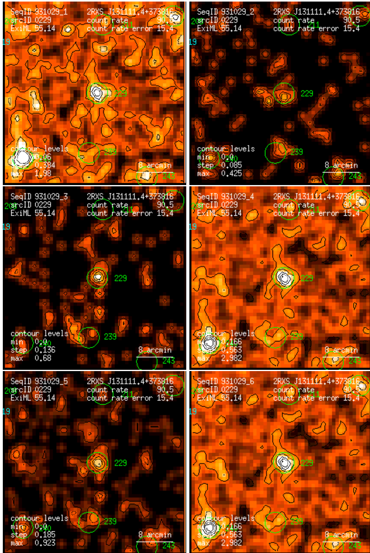
Figure 229: RASS 931029: detection 0229: band rate images, Gaussian filter: (1) PSPC channels 11 – 41, (2) 52 – 90, (3) 91 – 201, (4) 11 – 235, (5) 52 – 201, (6) 11 – 201. Broad band rates in counts/ks. Band rate contour levels in counts/ks/arcmin 2 .
