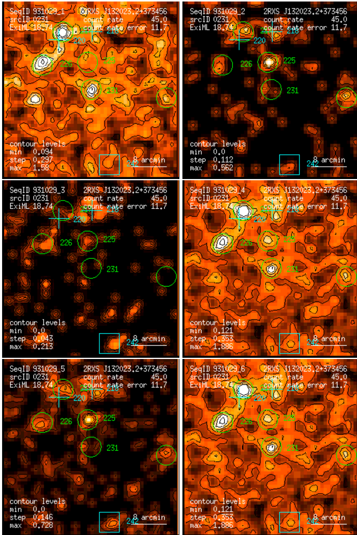
Figure 231: RASS 931029: detection 0231: band rate images, Gaussian filter: (1) PSPC channels 11 – 41, (2) 52 – 90, (3) 91 – 201, (4) 11 – 235, (5) 52 – 201, (6) 11 – 201. Broad band rates in counts/ks. Band rate contour levels in counts/ks/arcmin 2 .
