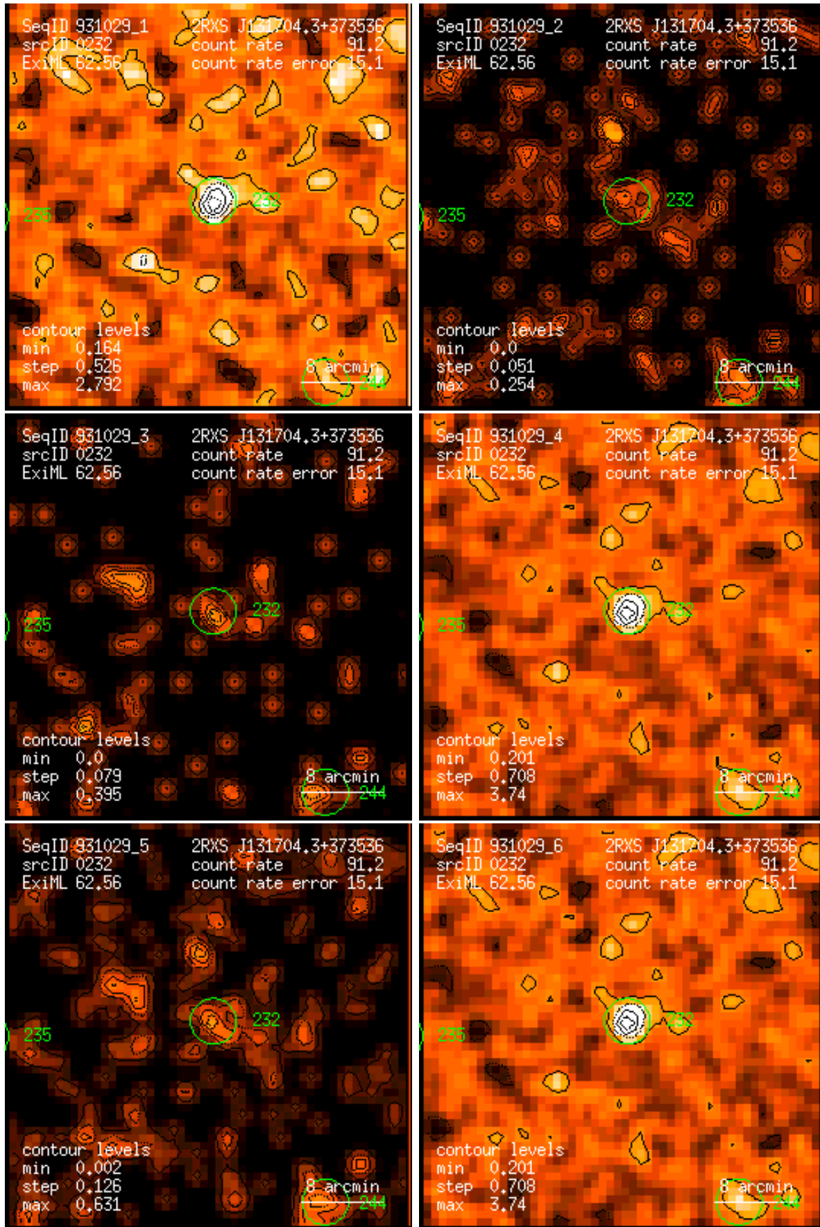
Figure 232: RASS 931029: detection 0232: band rate images, Gaussian filter: (1) PSPC channels 11 – 41, (2) 52 – 90, (3) 91 – 201, (4) 11 – 235, (5) 52 – 201, (6) 11 – 201. Broad band rates in counts/ks. Band rate contour levels in counts/ks/arcmin 2 .
