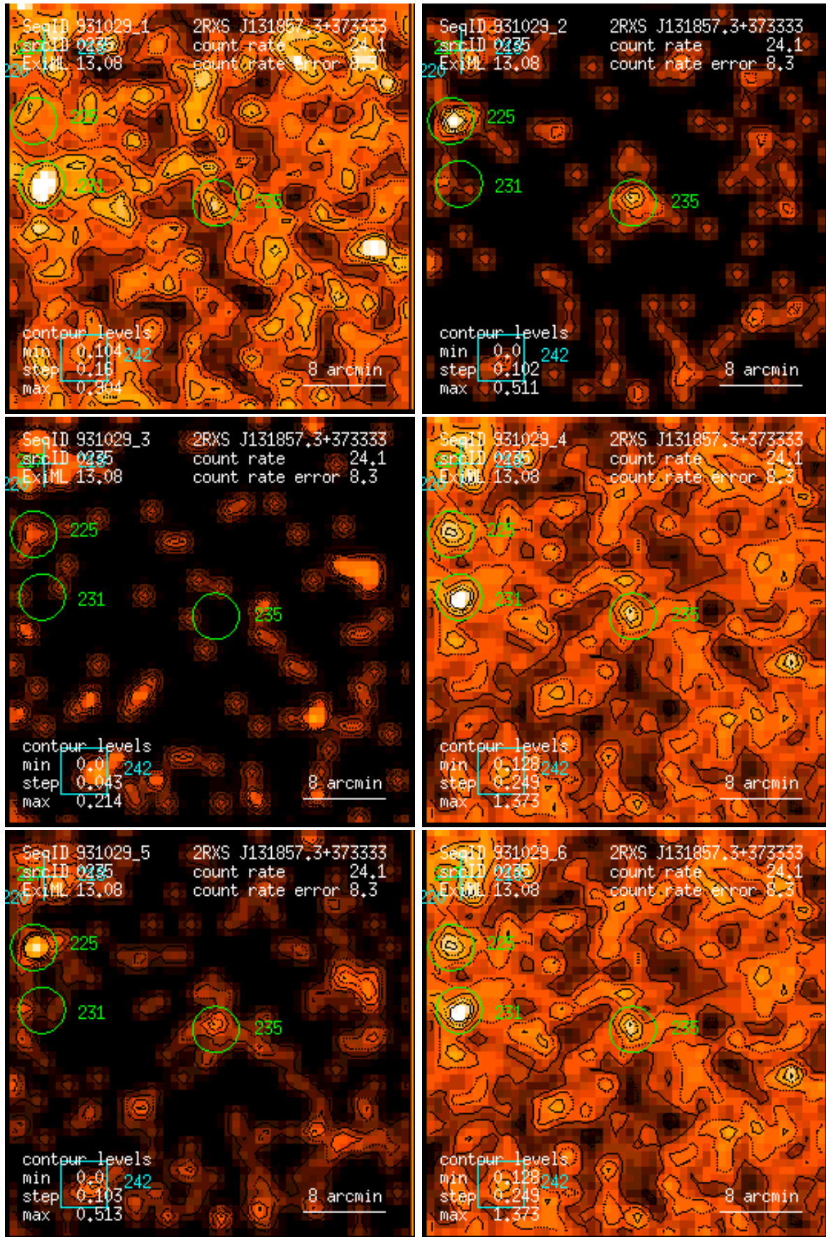
Figure 235: RASS 931029: detection 0235: band rate images, Gaussian filter: (1) PSPC channels 11 – 41, (2) 52 – 90, (3) 91 – 201, (4) 11 – 235, (5) 52 – 201, (6) 11 – 201. Broad band rates in counts/ks. Band rate contour levels in counts/ks/arcmin 2 .
