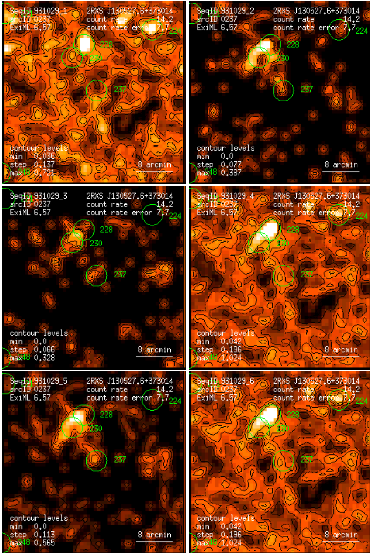
Figure 237: RASS 931029: detection 0237: band rate images, Gaussian filter: (1) PSPC channels 11 – 41, (2) 52 – 90, (3) 91 – 201, (4) 11 – 235, (5) 52 – 201, (6) 11 – 201. Broad band rates in counts/ks. Band rate contour levels in counts/ks/arcmin 2 .
