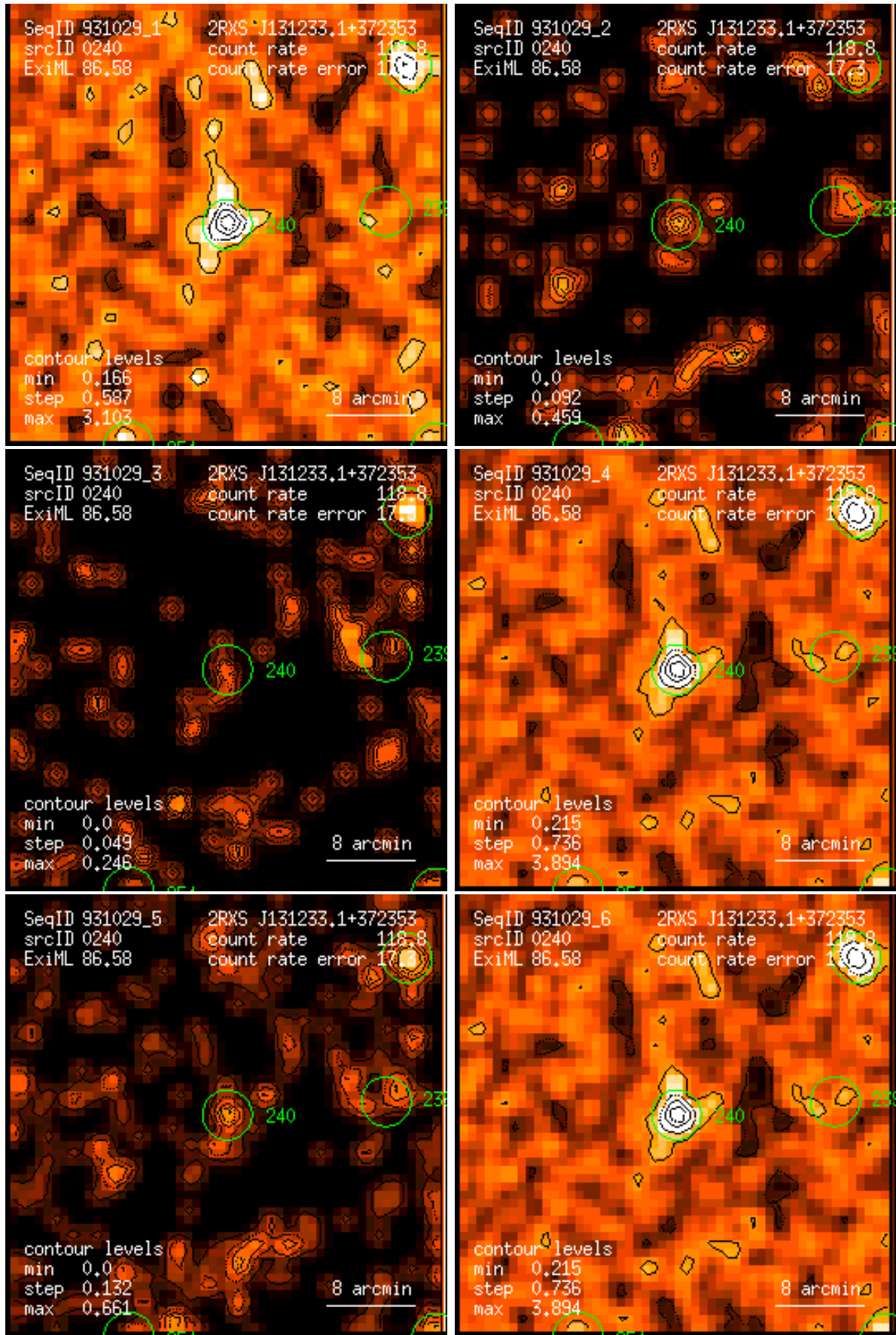
Figure 240: RASS 931029: detection 0240: band rate images, Gaussian filter: (1) PSPC channels 11 – 41, (2) 52 – 90, (3) 91 – 201, (4) 11 – 235, (5) 52 – 201, (6) 11 – 201. Broad band rates in counts/ks. Band rate contour levels in counts/ks/arcmin 2 .
