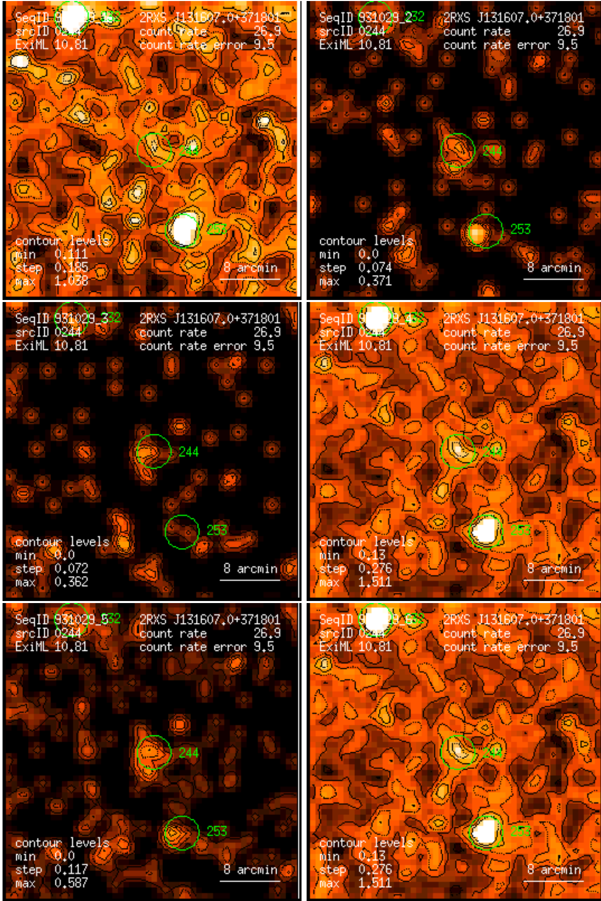
Figure 244: RASS 931029: detection 0244: band rate images, Gaussian filter: (1) PSPC channels 11 – 41, (2) 52 – 90, (3) 91 – 201, (4) 11 – 235, (5) 52 – 201, (6) 11 – 201. Broad band rates in counts/ks. Band rate contour levels in counts/ks/arcmin 2 .
