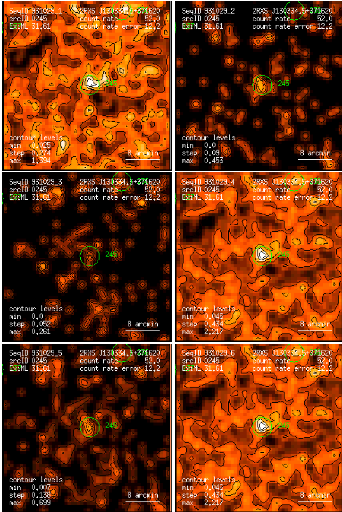
Figure 245: RASS 931029: detection 0245: band rate images, Gaussian filter: (1) PSPC channels 11 – 41, (2) 52 – 90, (3) 91 – 201, (4) 11 – 235, (5) 52 – 201, (6) 11 – 201. Broad band rates in counts/ks. Band rate contour levels in counts/ks/arcmin 2 .
