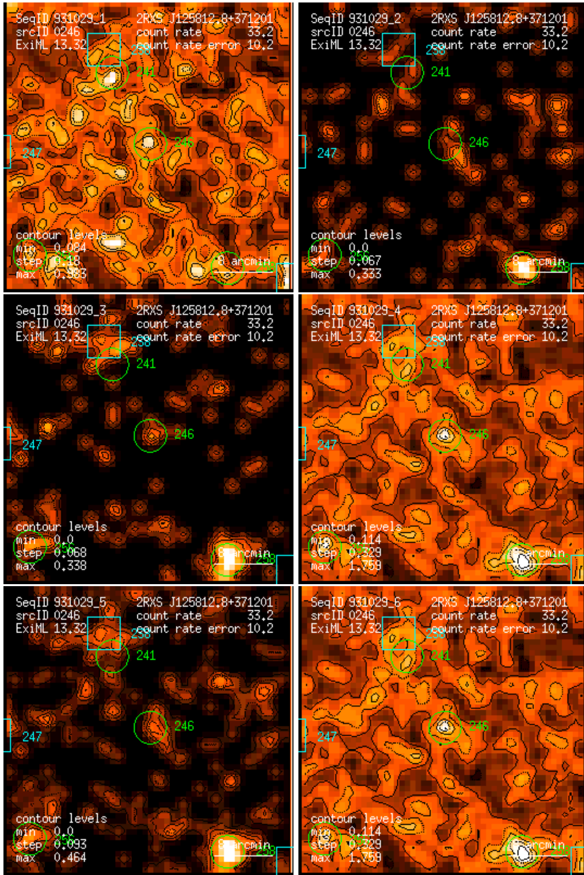
Figure 246: RASS 931029: detection 0246: band rate images, Gaussian filter: (1) PSPC channels 11 – 41, (2) 52 – 90, (3) 91 – 201, (4) 11 – 235, (5) 52 – 201, (6) 11 – 201. Broad band rates in counts/ks. Band rate contour levels in counts/ks/arcmin 2 .
