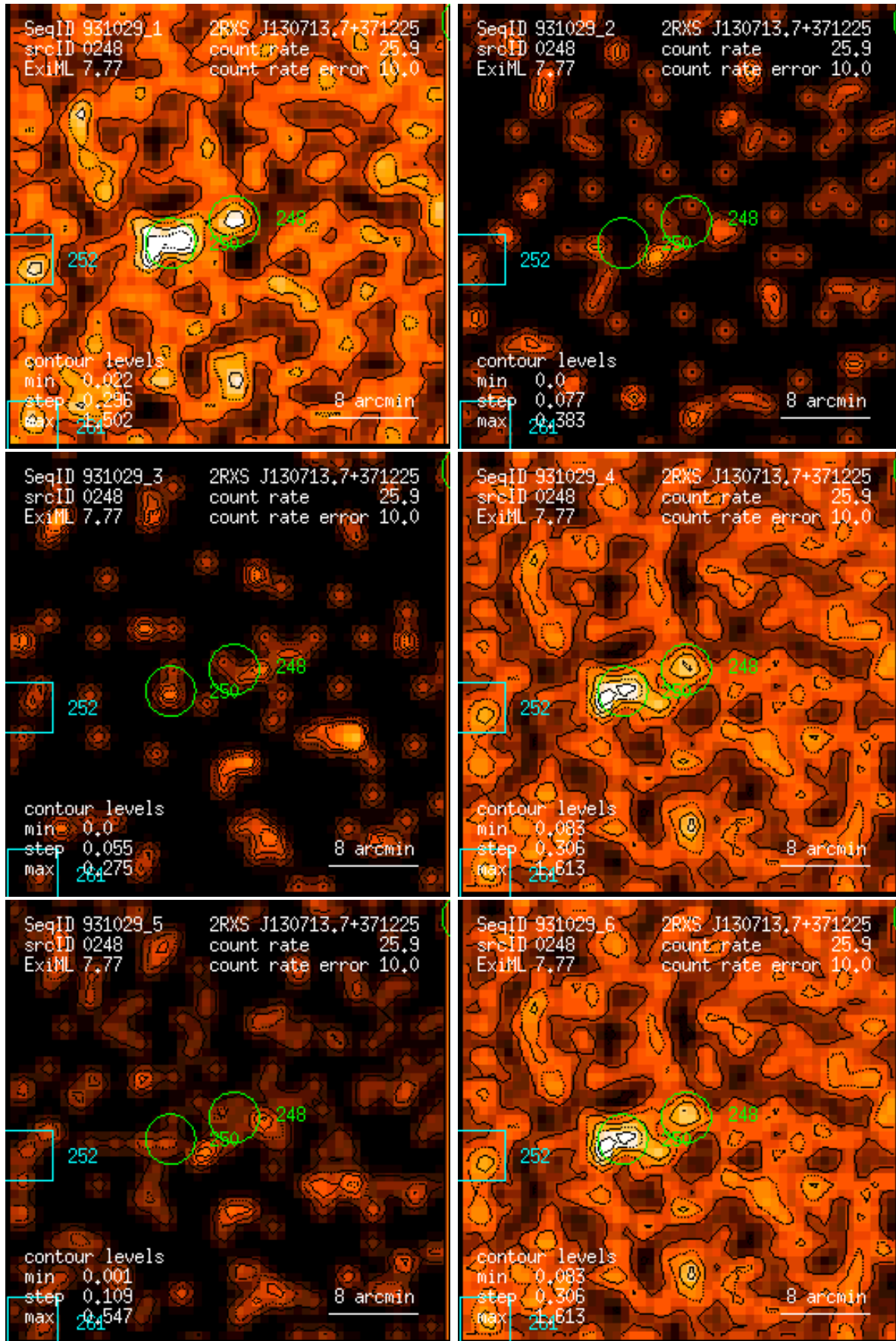
Figure 248: RASS 931029: detection 0248: band rate images, Gaussian filter: (1) PSPC channels 11 – 41, (2) 52 – 90, (3) 91 – 201, (4) 11 – 235, (5) 52 – 201, (6) 11 – 201. Broad band rates in counts/ks. Band rate contour levels in counts/ks/arcmin 2 .
