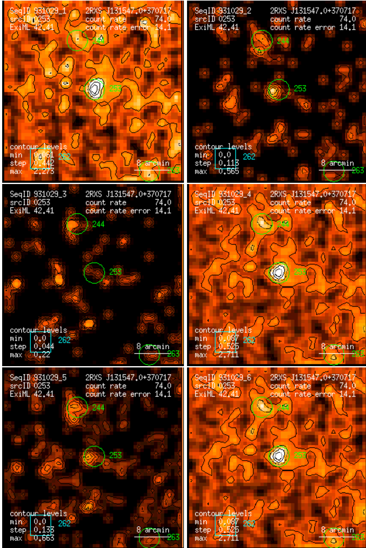
Figure 253: RASS 931029: detection 0253: band rate images, Gaussian filter: (1) PSPC channels 11 – 41, (2) 52 – 90, (3) 91 – 201, (4) 11 – 235, (5) 52 – 201, (6) 11 – 201. Broad band rates in counts/ks. Band rate contour levels in counts/ks/arcmin 2 .
