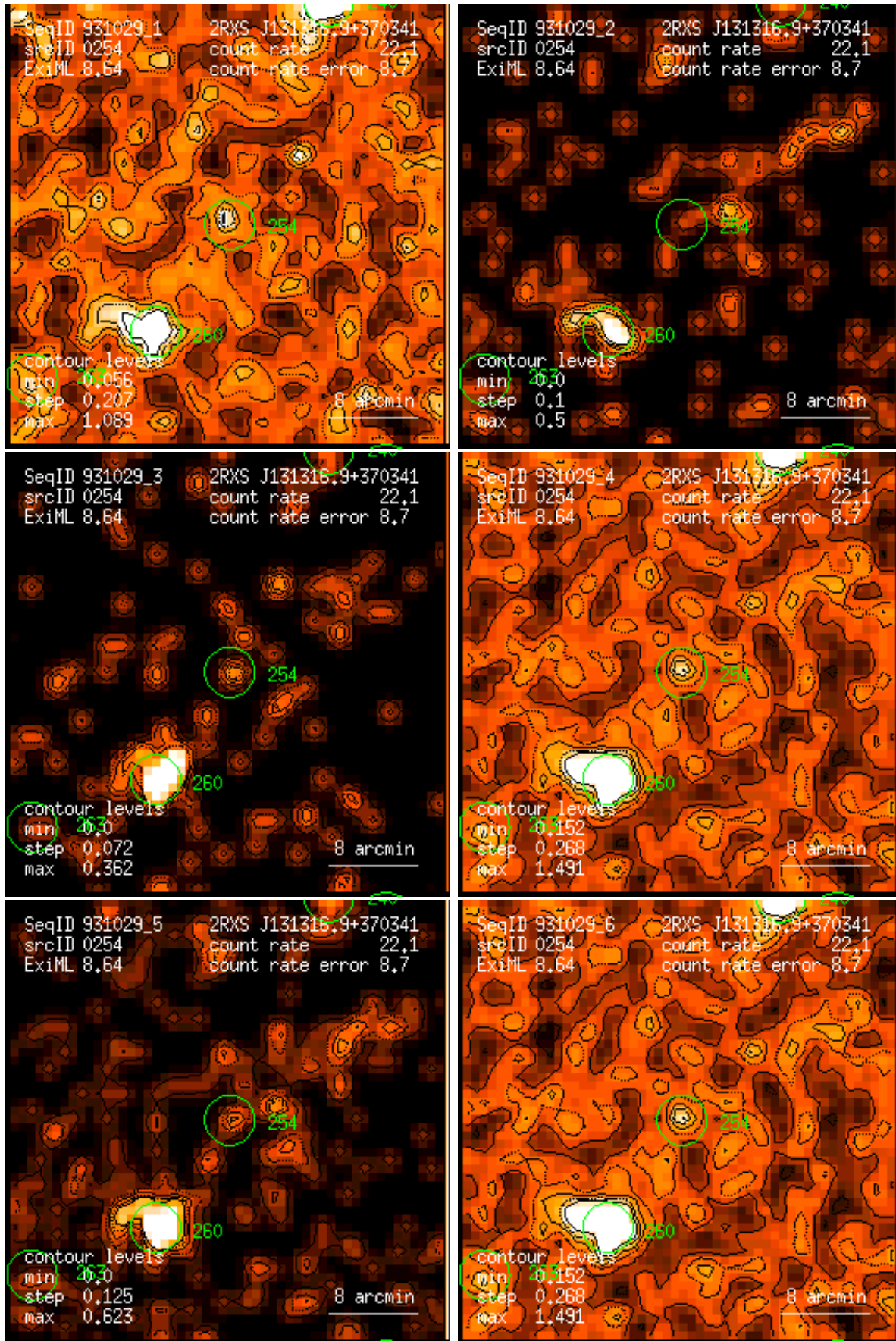
Figure 254: RASS 931029: detection 0254: band rate images, Gaussian filter: (1) PSPC channels 11 – 41, (2) 52 – 90, (3) 91 – 201, (4) 11 – 235, (5) 52 – 201, (6) 11 – 201. Broad band rates in counts/ks. Band rate contour levels in counts/ks/arcmin 2 .
