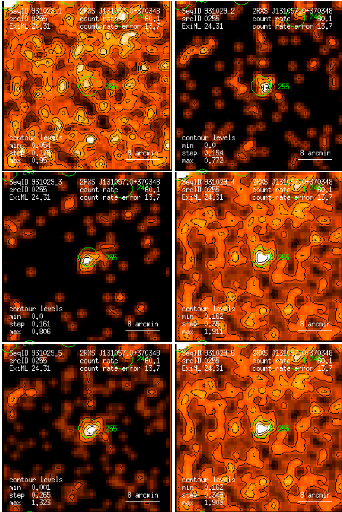
Figure 255: RASS 931029: detection 0255: band rate images, Gaussian filter: (1) PSPC channels 11 – 41, (2) 52 – 90, (3) 91 – 201, (4) 11 – 235, (5) 52 – 201, (6) 11 – 201. Broad band rates in counts/ks. Band rate contour levels in counts/ks/arcmin 2 .
