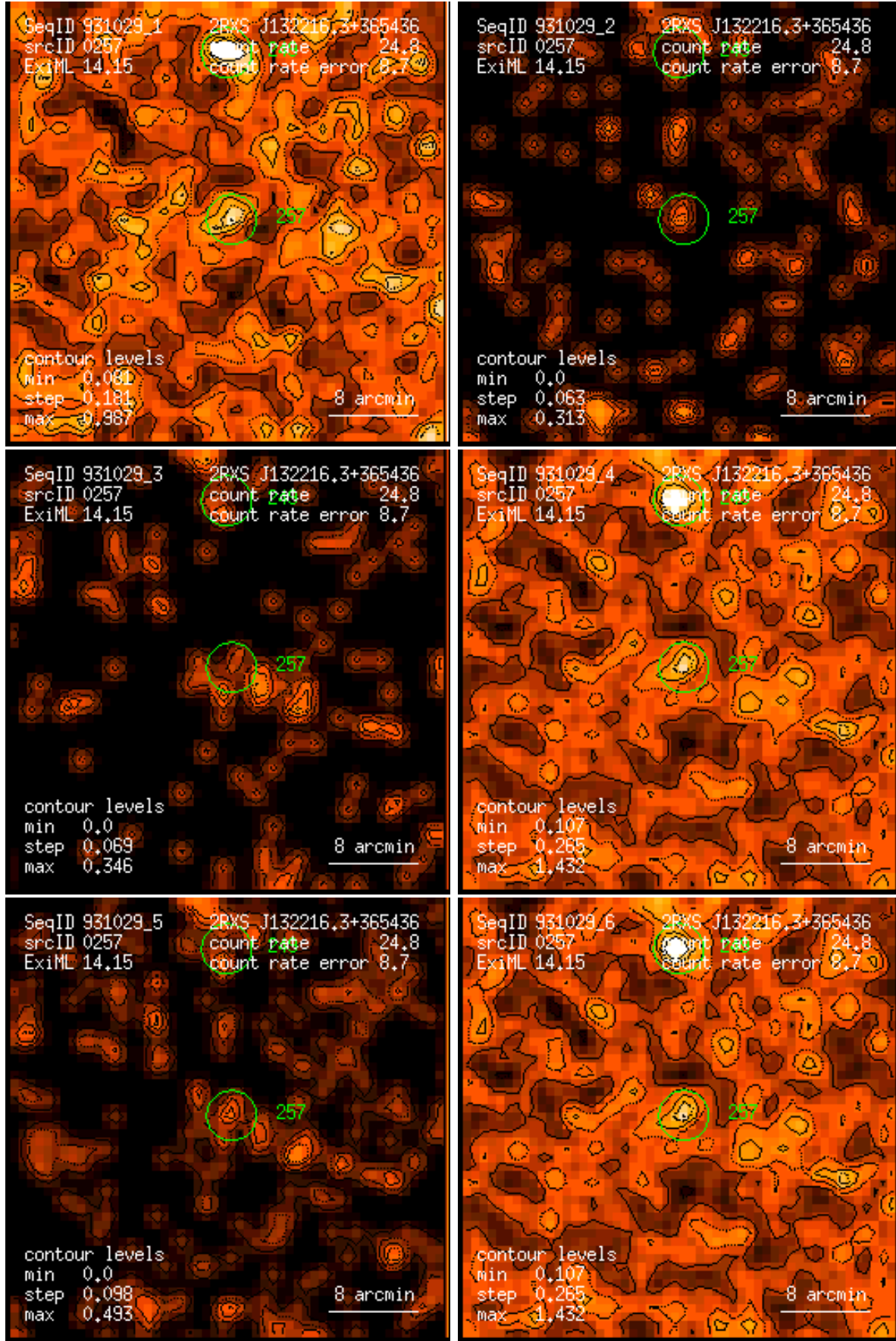
Figure 257: RASS 931029: detection 0257: band rate images, Gaussian filter: (1) PSPC channels 11 – 41, (2) 52 – 90, (3) 91 – 201, (4) 11 – 235, (5) 52 – 201, (6) 11 – 201. Broad band rates in counts/ks. Band rate contour levels in counts/ks/arcmin 2 .
