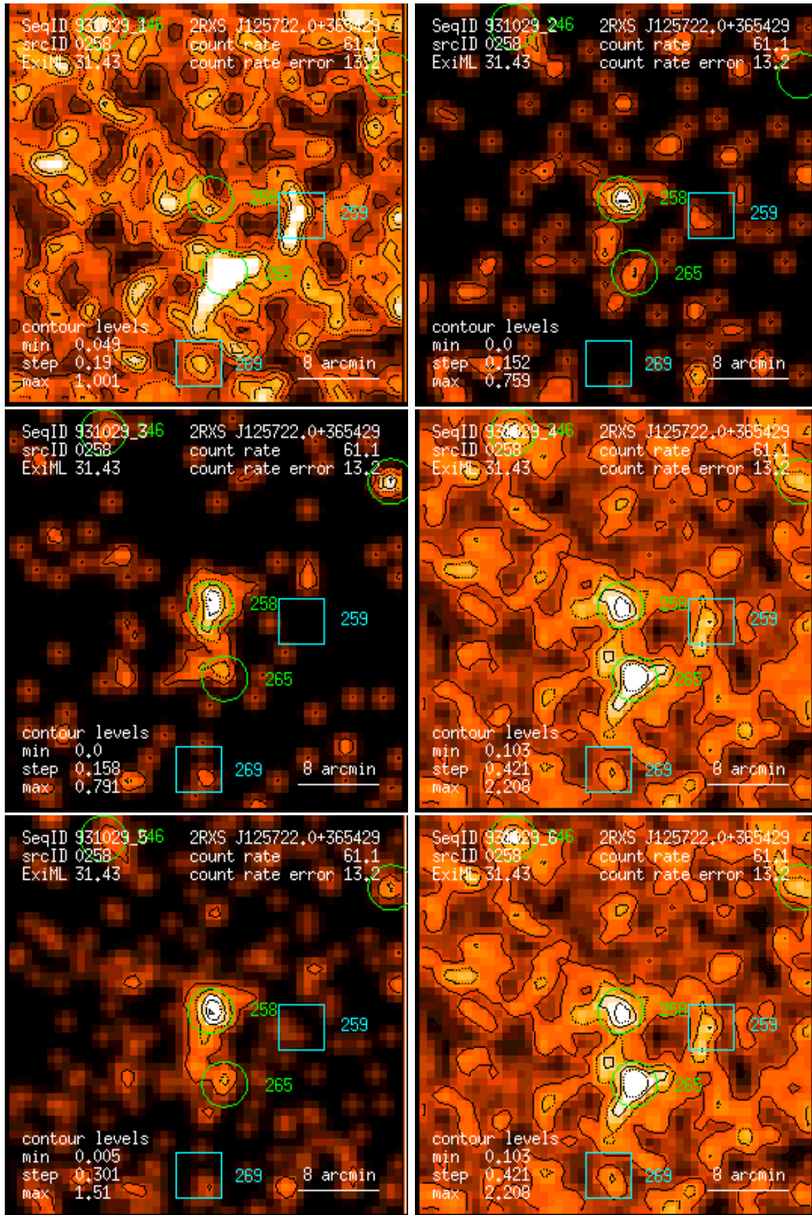
Figure 258: RASS 931029: detection 0258: band rate images, Gaussian filter: (1) PSPC channels 11 – 41, (2) 52 – 90, (3) 91 – 201, (4) 11 – 235, (5) 52 – 201, (6) 11 – 201. Broad band rates in counts/ks. Band rate contour levels in counts/ks/arcmin 2 .
