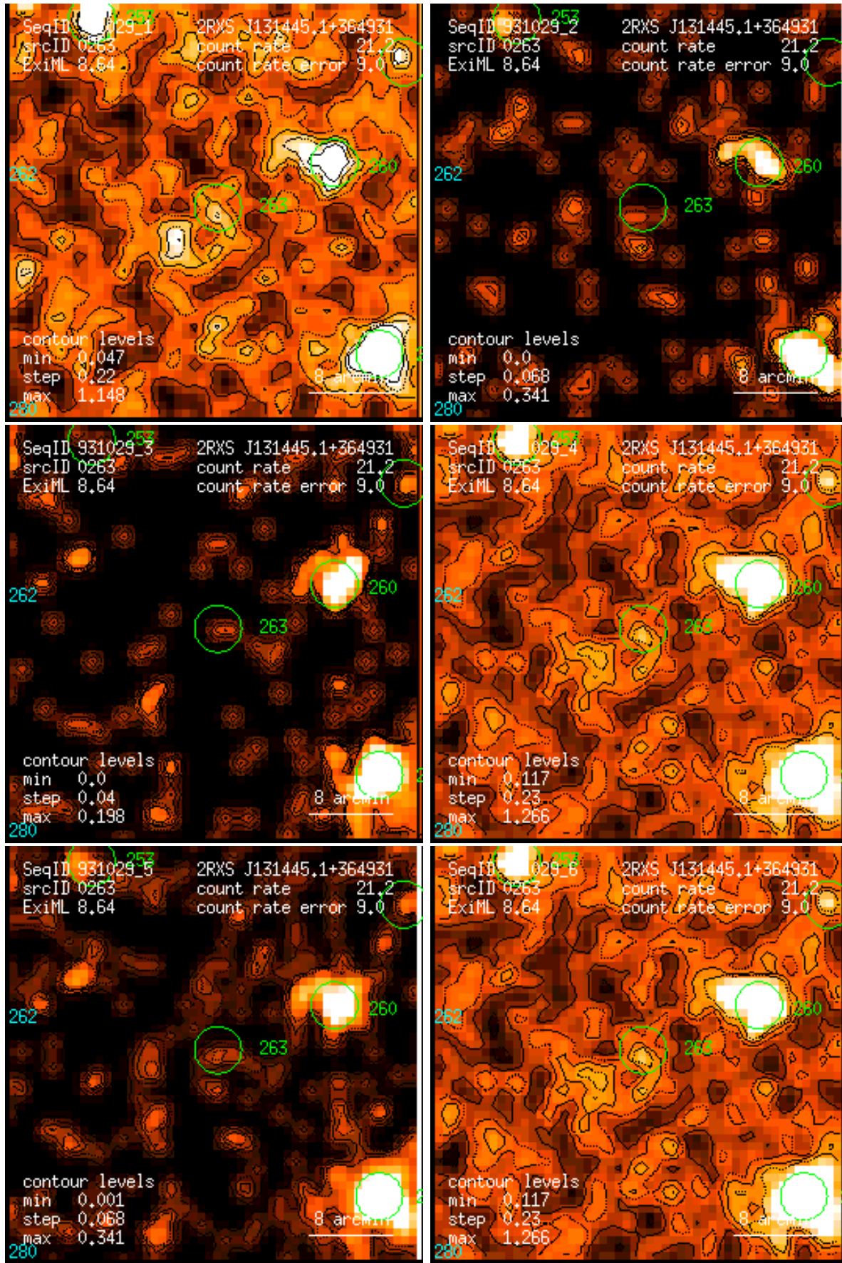
Figure 263: RASS 931029: detection 0263: band rate images, Gaussian filter: (1) PSPC channels 11 – 41, (2) 52 – 90, (3) 91 – 201, (4) 11 – 235, (5) 52 – 201, (6) 11 – 201. Broad band rates in counts/ks. Band rate contour levels in counts/ks/arcmin 2 .
