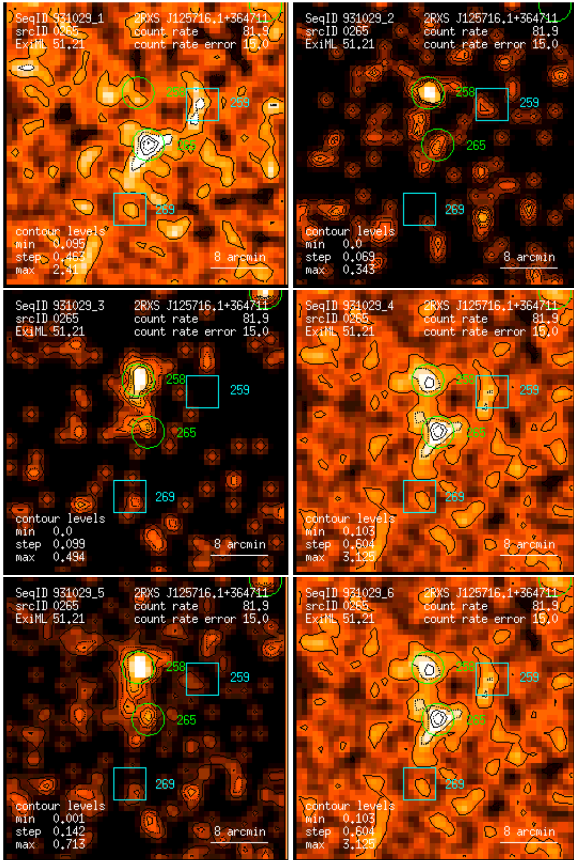
Figure 265: RASS 931029: detection 0265: band rate images, Gaussian filter: (1) PSPC channels 11 – 41, (2) 52 – 90, (3) 91 – 201, (4) 11 – 235, (5) 52 – 201, (6) 11 – 201. Broad band rates in counts/ks. Band rate contour levels in counts/ks/arcmin 2 .
