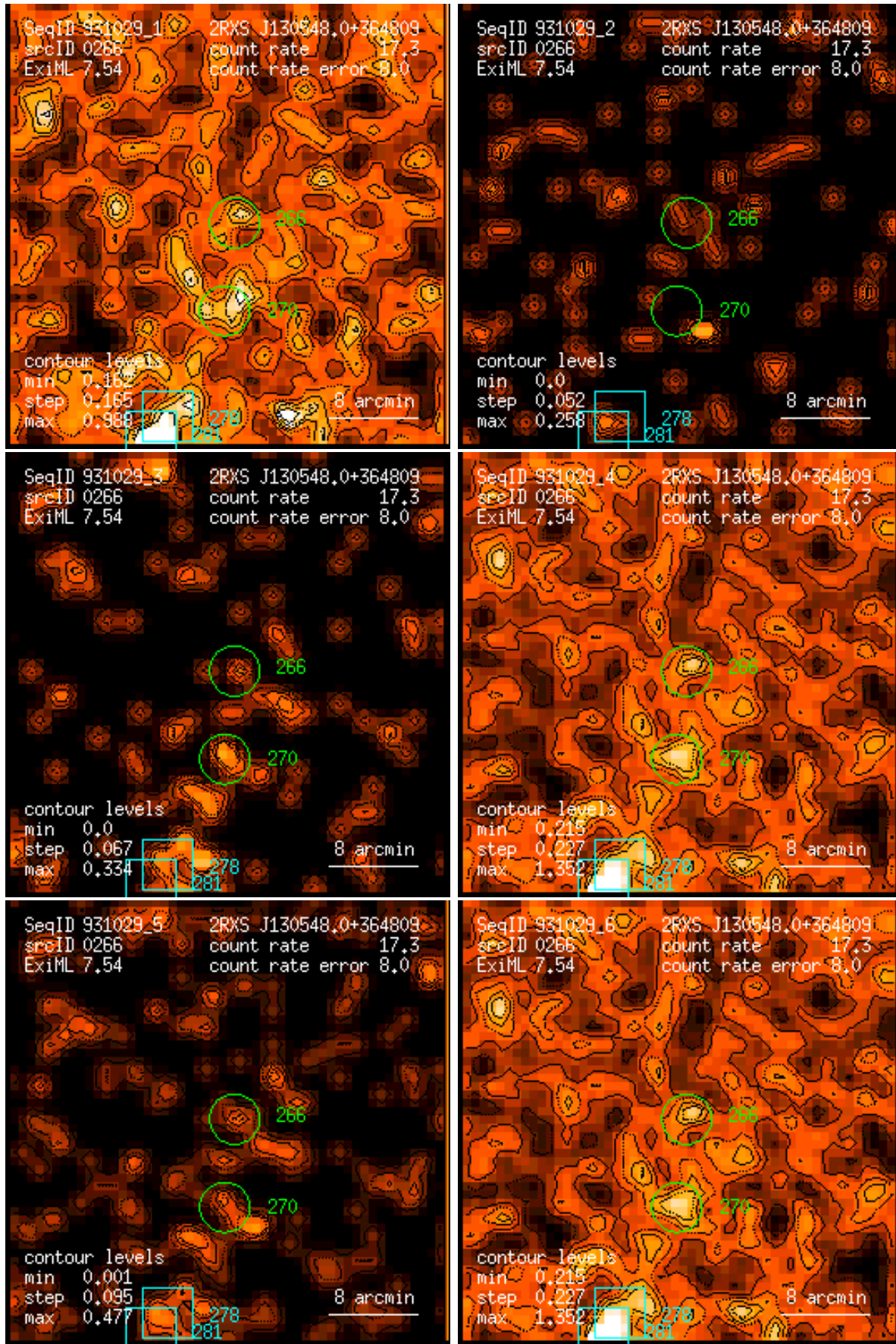
Figure 266: RASS 931029: detection 0266: band rate images, Gaussian filter: (1) PSPC channels 11 – 41, (2) 52 – 90, (3) 91 – 201, (4) 11 – 235, (5) 52 – 201, (6) 11 – 201. Broad band rates in counts/ks. Band rate contour levels in counts/ks/arcmin 2 .
