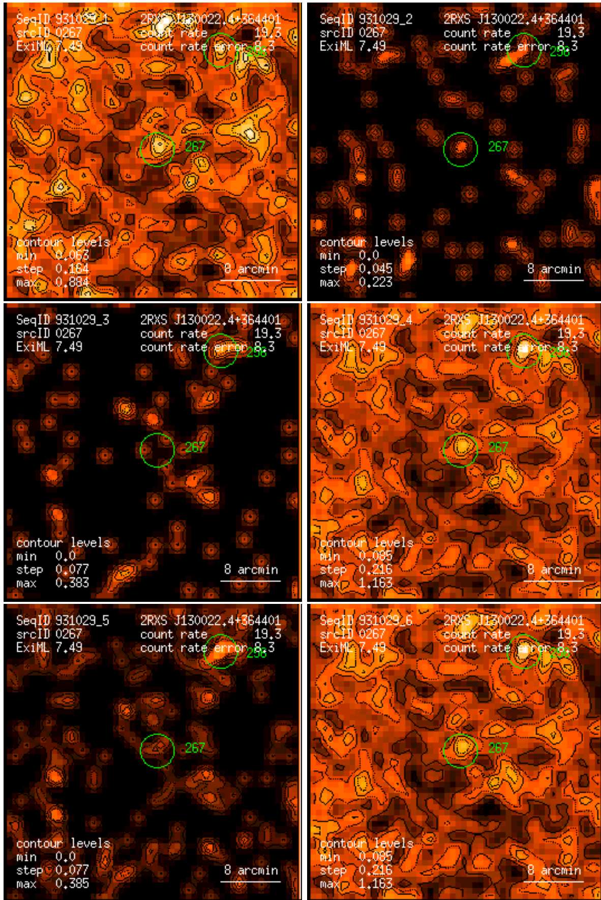
Figure 267: RASS 931029: detection 0267: band rate images, Gaussian filter: (1) PSPC channels 11 – 41, (2) 52 – 90, (3) 91 – 201, (4) 11 – 235, (5) 52 – 201, (6) 11 – 201. Broad band rates in counts/ks. Band rate contour levels in counts/ks/arcmin 2 .
