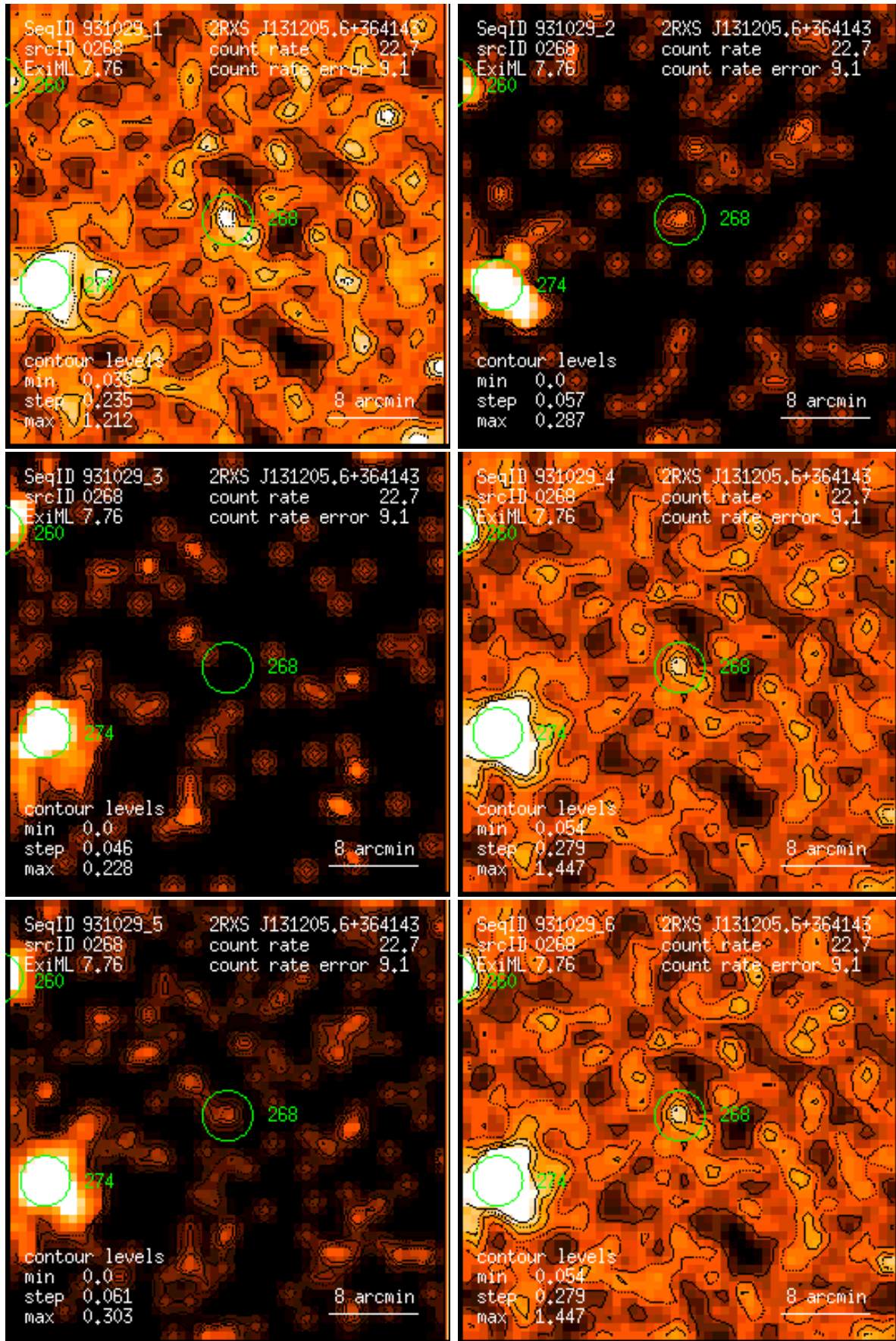
Figure 268: RASS 931029: detection 0268: band rate images, Gaussian filter: (1) PSPC channels 11 – 41, (2) 52 – 90, (3) 91 – 201, (4) 11 – 235, (5) 52 – 201, (6) 11 – 201. Broad band rates in counts/ks. Band rate contour levels in counts/ks/arcmin 2 .
