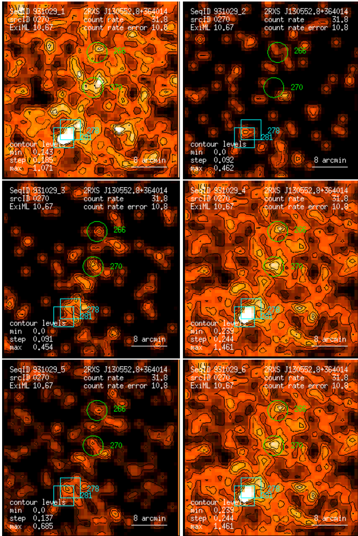
Figure 270: RASS 931029: detection 0270: band rate images, Gaussian filter: (1) PSPC channels 11 – 41, (2) 52 – 90, (3) 91 – 201, (4) 11 – 235, (5) 52 – 201, (6) 11 – 201. Broad band rates in counts/ks. Band rate contour levels in counts/ks/arcmin 2 .
