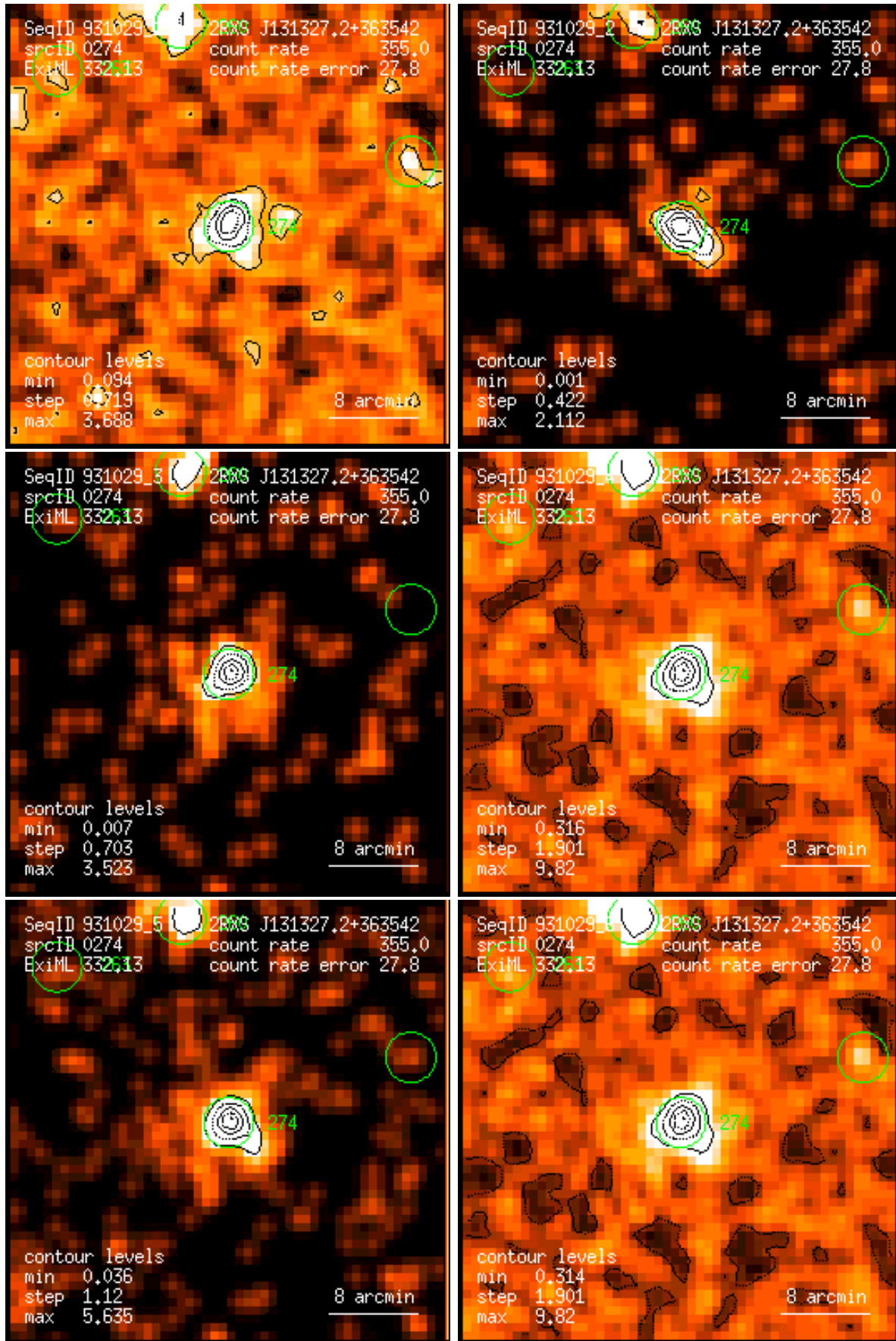
Figure 274: RASS 931029: detection 0274: band rate images, Gaussian filter: (1) PSPC channels 11 – 41, (2) 52 – 90, (3) 91 – 201, (4) 11 – 235, (5) 52 – 201, (6) 11 – 201. Broad band rates in counts/ks. Band rate contour levels in counts/ks/arcmin 2 .
