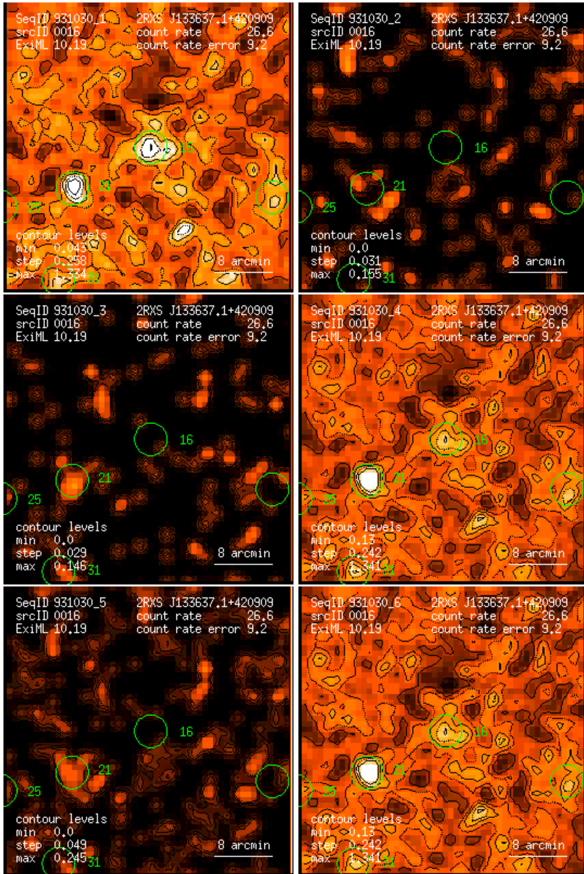
Figure 16: RASS 931030: detection 0016: band rate images, Gaussian filter: (1) PSPC channels 11 – 41, (2) 52 – 90, (3) 91 – 201, (4) 11 – 235, (5) 52 – 201, (6) 11 – 201. Broad band rates in counts/ks. Band rate contour levels in counts/ks/arcmin 2 .
