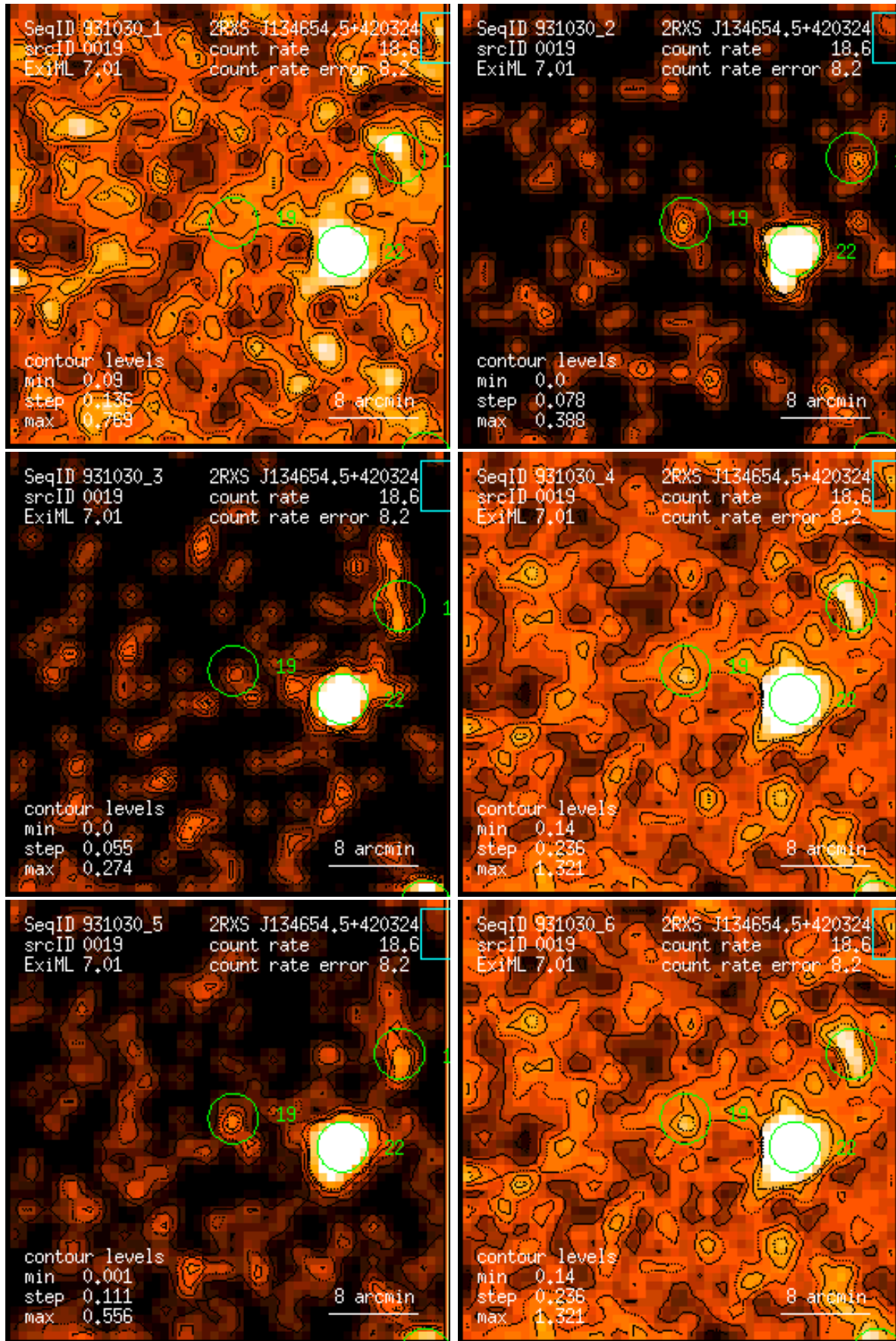
Figure 19: RASS 931030: detection 0019: band rate images, Gaussian filter: (1) PSPC channels 11 – 41, (2) 52 – 90, (3) 91 – 201, (4) 11 – 235, (5) 52 – 201, (6) 11 – 201. Broad band rates in counts/ks. Band rate contour levels in counts/ks/arcmin 2 .
