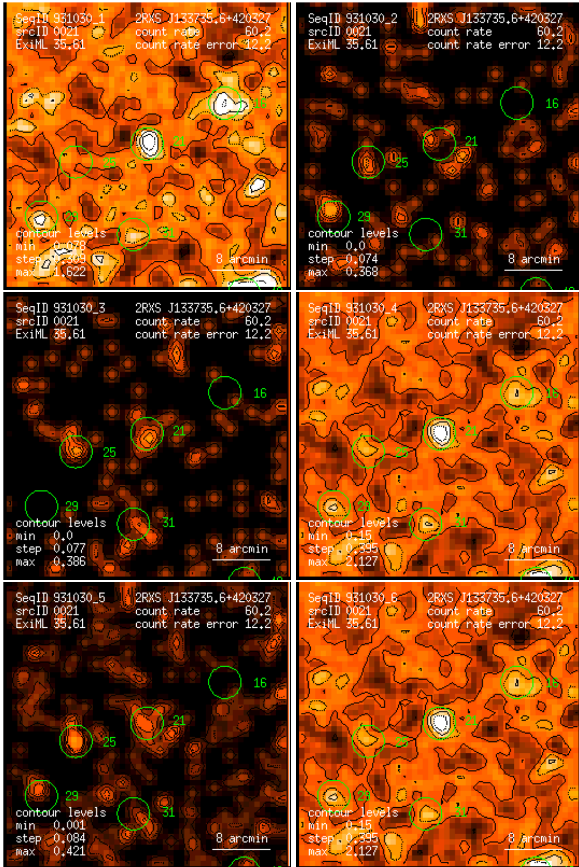
Figure 21: RASS 931030: detection 0021: band rate images, Gaussian filter: (1) PSPC channels 11 – 41, (2) 52 – 90, (3) 91 – 201, (4) 11 – 235, (5) 52 – 201, (6) 11 – 201. Broad band rates in counts/ks. Band rate contour levels in counts/ks/arcmin 2 .
