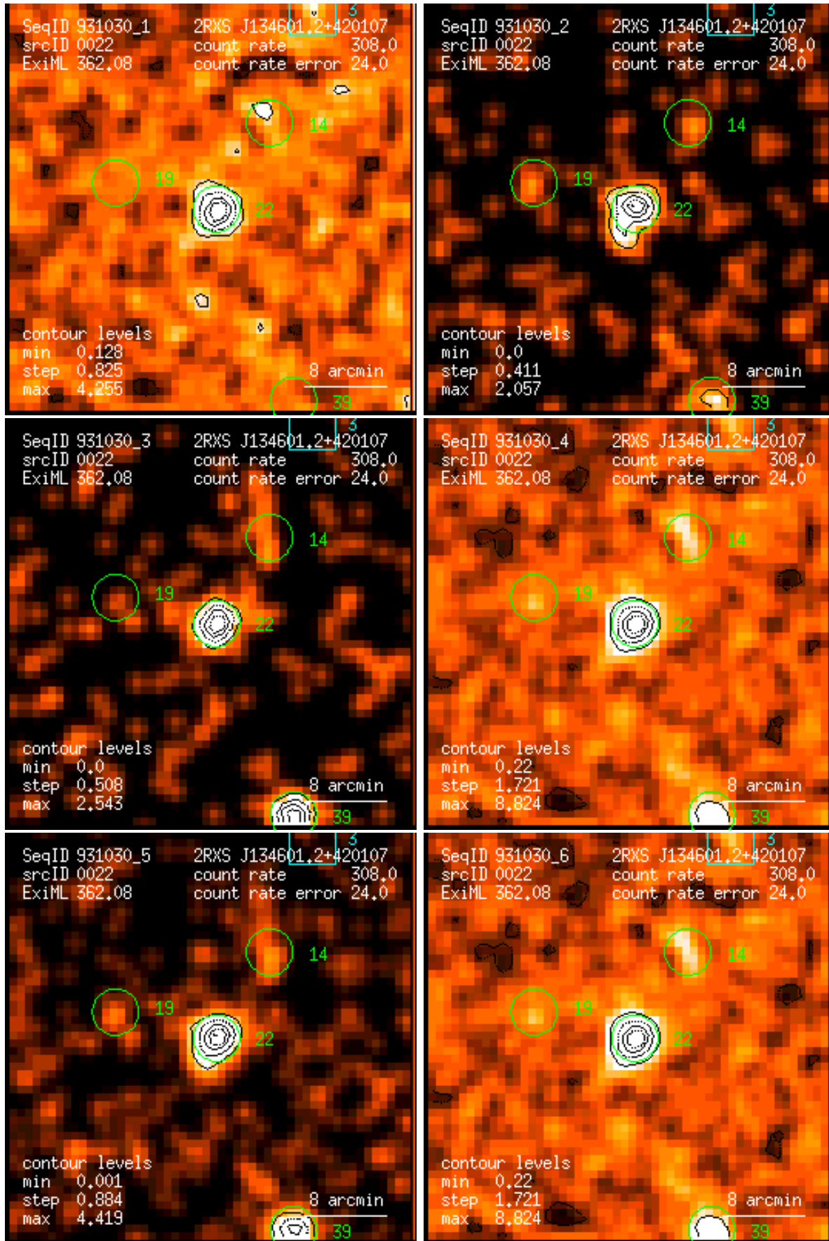
Figure 22: RASS 931030: detection 0022: band rate images, Gaussian filter: (1) PSPC channels 11 – 41, (2) 52 – 90, (3) 91 – 201, (4) 11 – 235, (5) 52 – 201, (6) 11 – 201. Broad band rates in counts/ks. Band rate contour levels in counts/ks/arcmin 2 .
