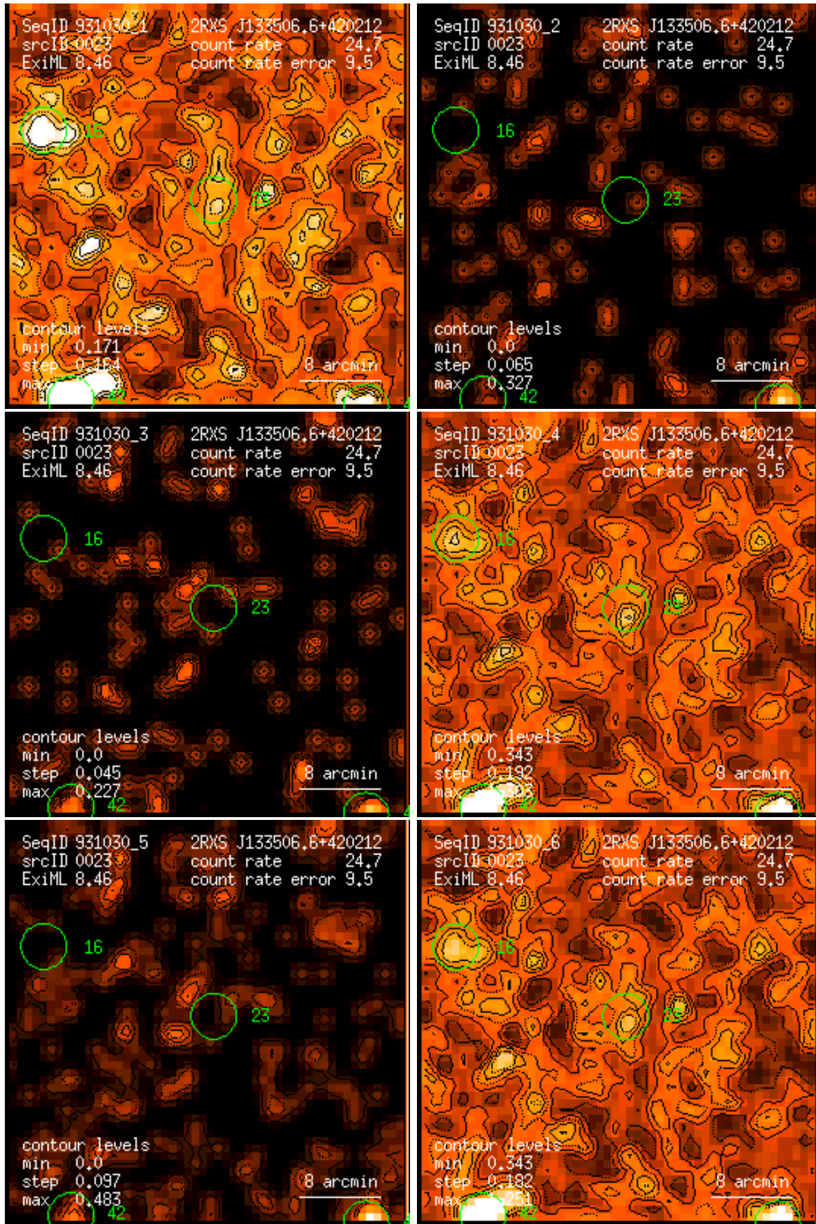
Figure 23: RASS 931030: detection 0023: band rate images, Gaussian filter: (1) PSPC channels 11 – 41, (2) 52 – 90, (3) 91 – 201, (4) 11 – 235, (5) 52 – 201, (6) 11 – 201. Broad band rates in counts/ks. Band rate contour levels in counts/ks/arcmin 2 .
