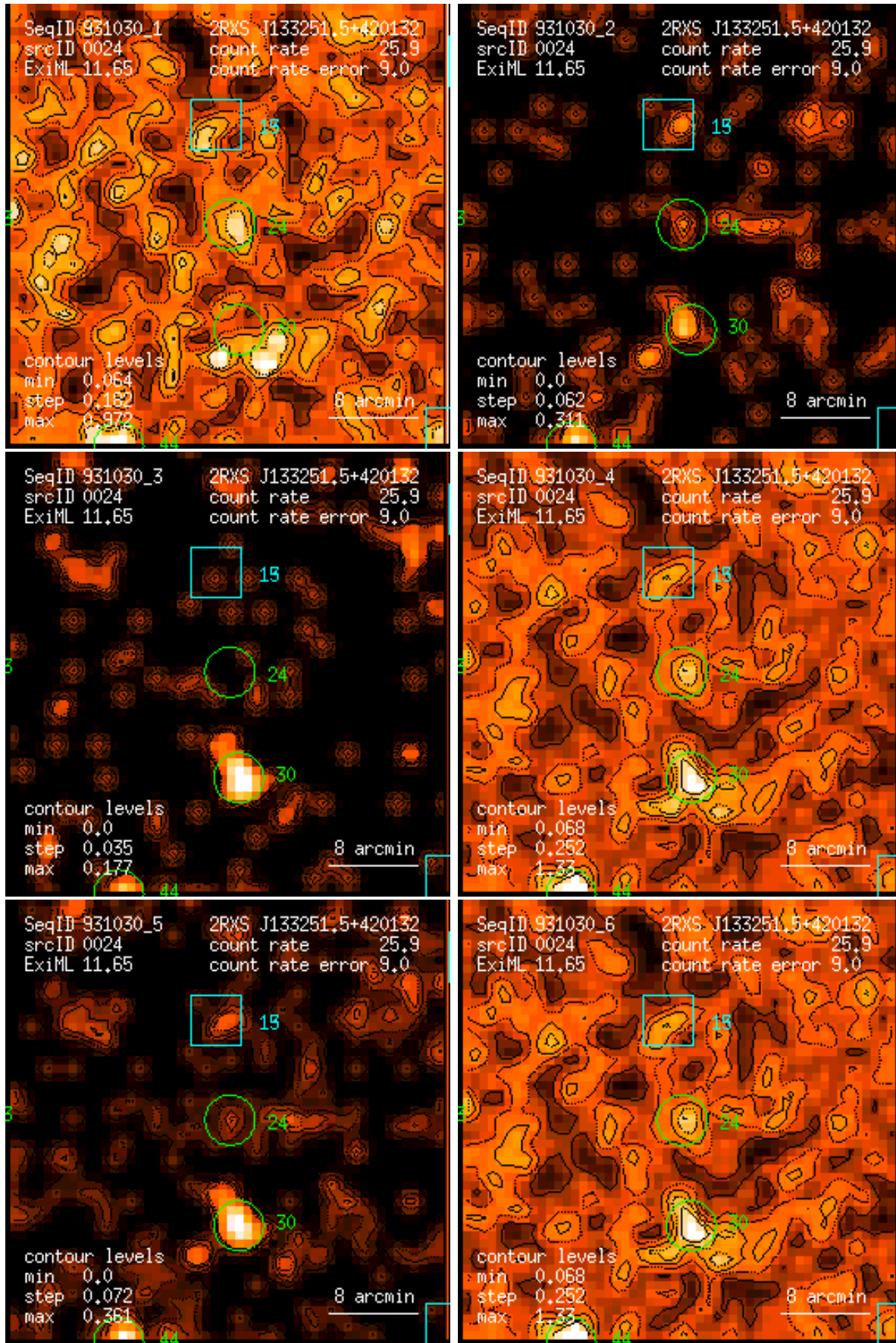
Figure 24: RASS 931030: detection 0024: band rate images, Gaussian filter: (1) PSPC channels 11 – 41, (2) 52 – 90, (3) 91 – 201, (4) 11 – 235, (5) 52 – 201, (6) 11 – 201. Broad band rates in counts/ks. Band rate contour levels in counts/ks/arcmin 2 .
