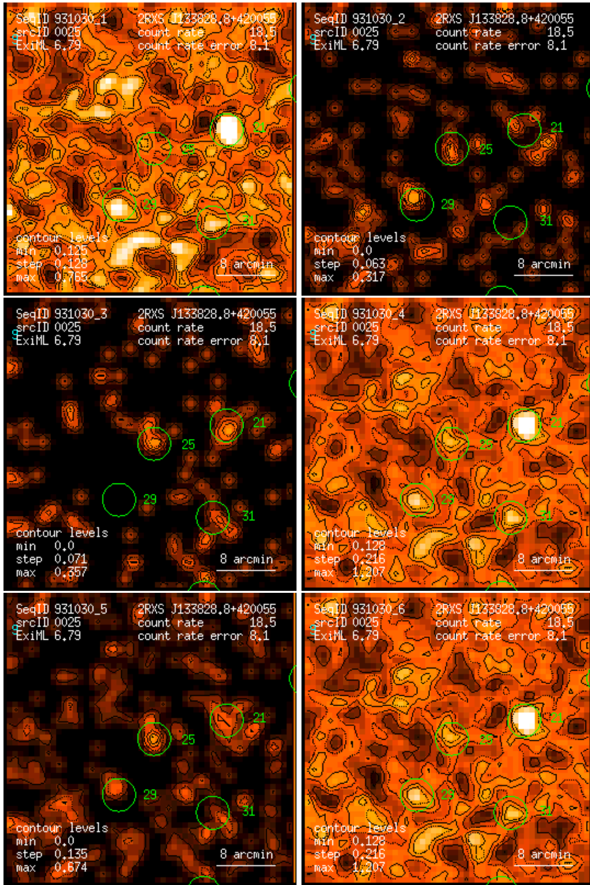
Figure 25: RASS 931030: detection 0025: band rate images, Gaussian filter: (1) PSPC channels 11 – 41, (2) 52 – 90, (3) 91 – 201, (4) 11 – 235, (5) 52 – 201, (6) 11 – 201. Broad band rates in counts/ks. Band rate contour levels in counts/ks/arcmin 2 .
