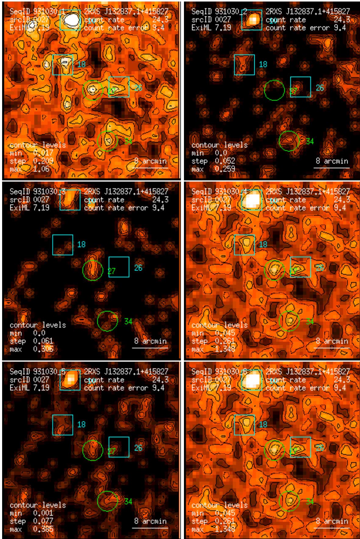
Figure 27: RASS 931030: detection 0027: band rate images, Gaussian filter: (1) PSPC channels 11 – 41, (2) 52 – 90, (3) 91 – 201, (4) 11 – 235, (5) 52 – 201, (6) 11 – 201. Broad band rates in counts/ks. Band rate contour levels in counts/ks/arcmin 2 .
