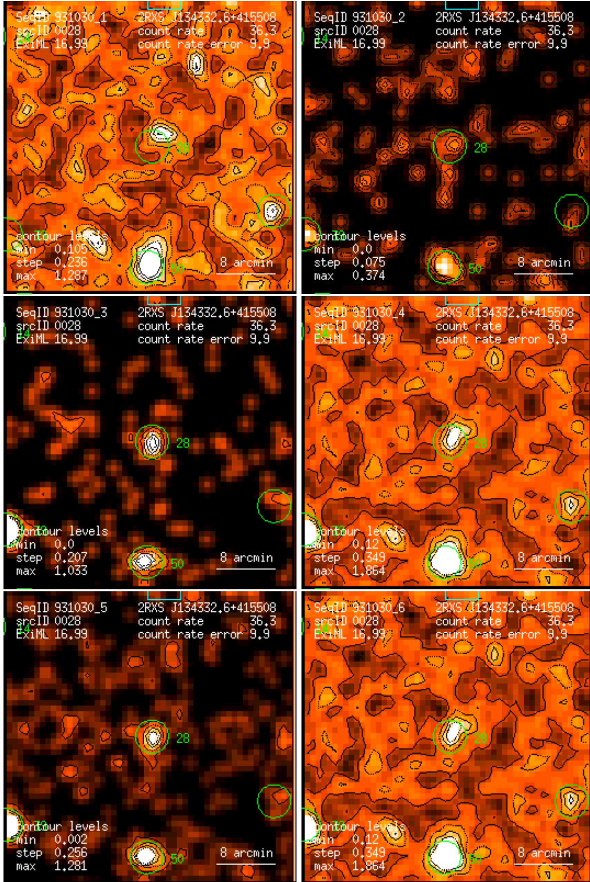
Figure 28: RASS 931030: detection 0028: band rate images, Gaussian filter: (1) PSPC channels 11 – 41, (2) 52 – 90, (3) 91 – 201, (4) 11 – 235, (5) 52 – 201, (6) 11 – 201. Broad band rates in counts/ks. Band rate contour levels in counts/ks/arcmin 2 .
