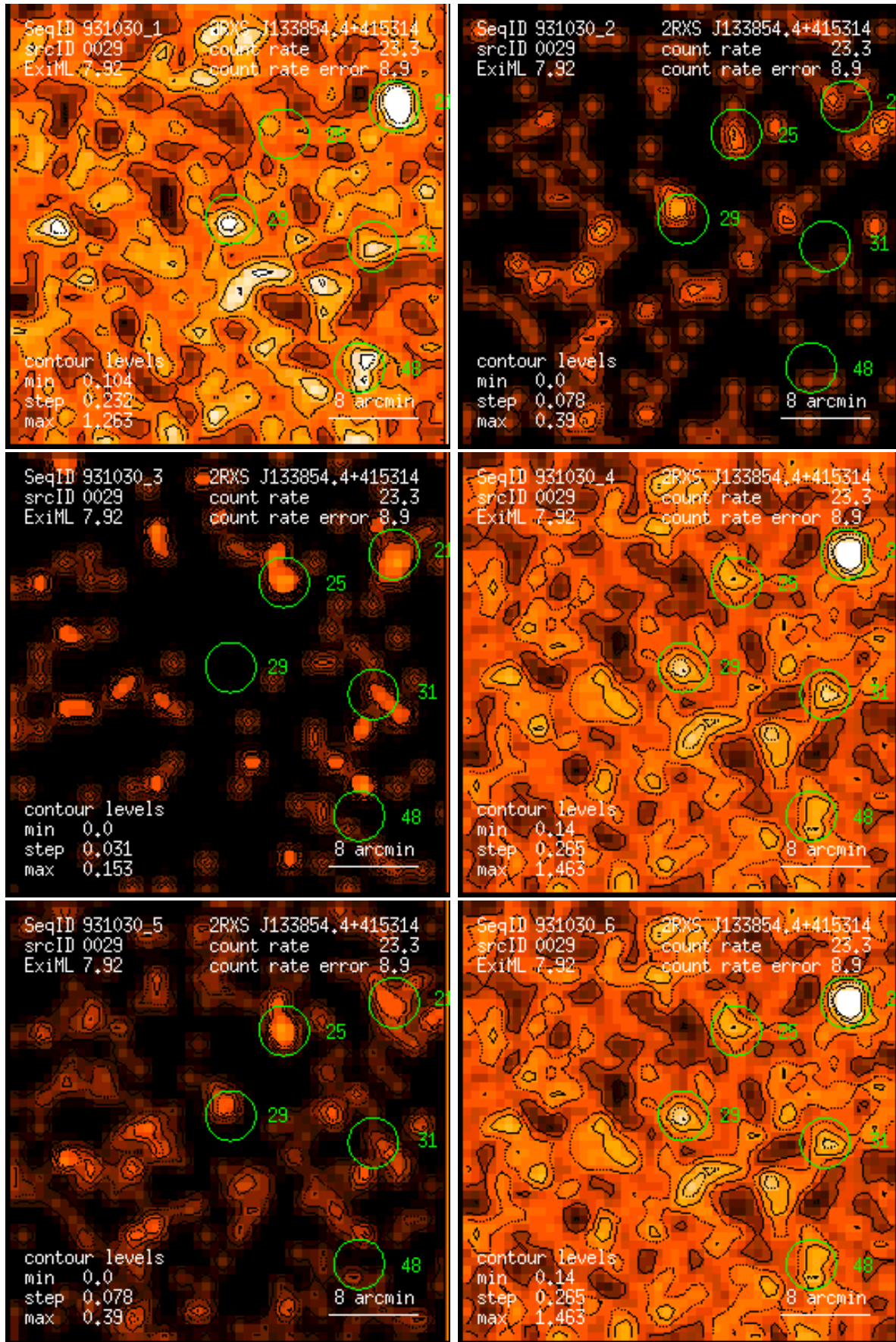
Figure 29: RASS 931030: detection 0029: band rate images, Gaussian filter: (1) PSPC channels 11 – 41, (2) 52 – 90, (3) 91 – 201, (4) 11 – 235, (5) 52 – 201, (6) 11 – 201. Broad band rates in counts/ks. Band rate contour levels in counts/ks/arcmin 2 .
