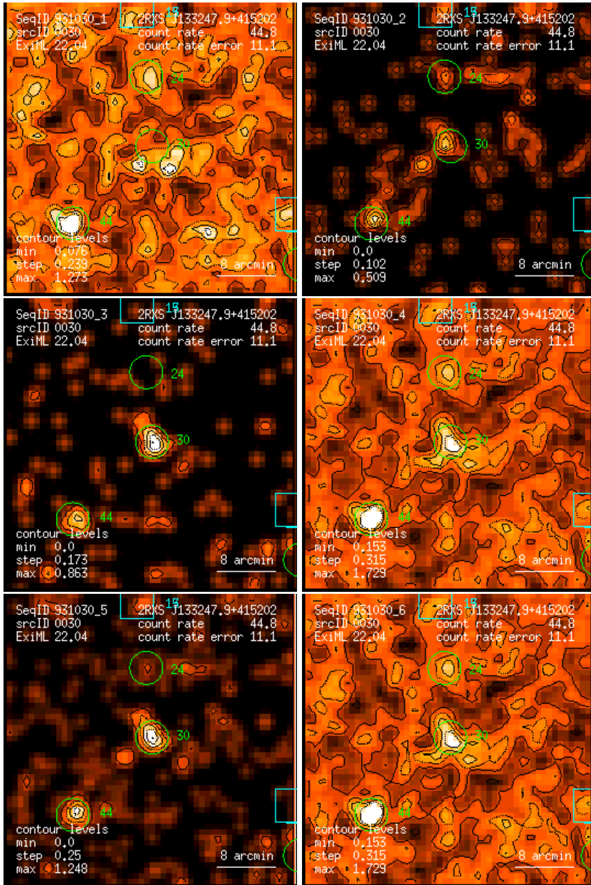
Figure 30: RASS 931030: detection 0030: band rate images, Gaussian filter: (1) PSPC channels 11 – 41, (2) 52 – 90, (3) 91 – 201, (4) 11 – 235, (5) 52 – 201, (6) 11 – 201. Broad band rates in counts/ks. Band rate contour levels in counts/ks/arcmin 2 .
