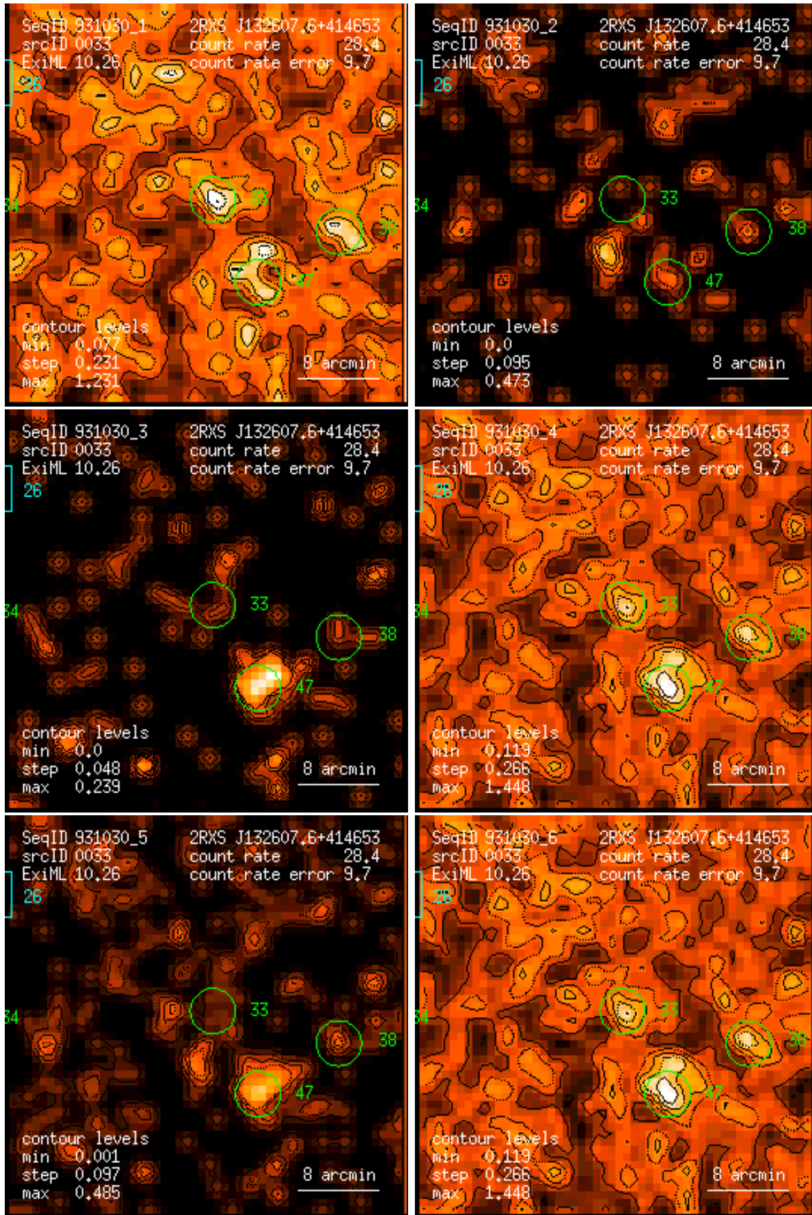
Figure 33: RASS 931030: detection 0033: band rate images, Gaussian filter: (1) PSPC channels 11 – 41, (2) 52 – 90, (3) 91 – 201, (4) 11 – 235, (5) 52 – 201, (6) 11 – 201. Broad band rates in counts/ks. Band rate contour levels in counts/ks/arcmin 2 .
