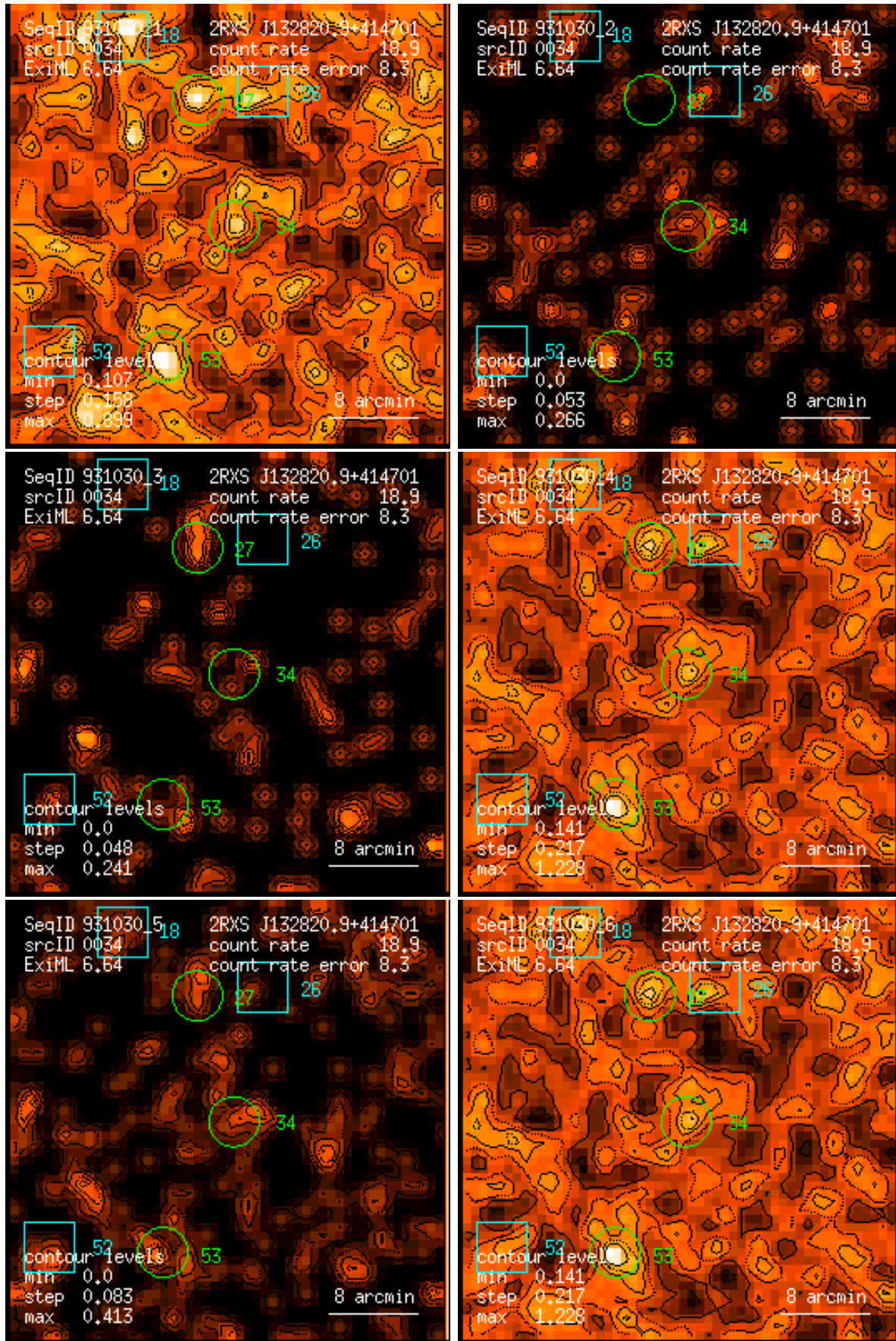
Figure 34: RASS 931030: detection 0034: band rate images, Gaussian filter: (1) PSPC channels 11 – 41, (2) 52 – 90, (3) 91 – 201, (4) 11 – 235, (5) 52 – 201, (6) 11 – 201. Broad band rates in counts/ks. Band rate contour levels in counts/ks/arcmin 2 .
