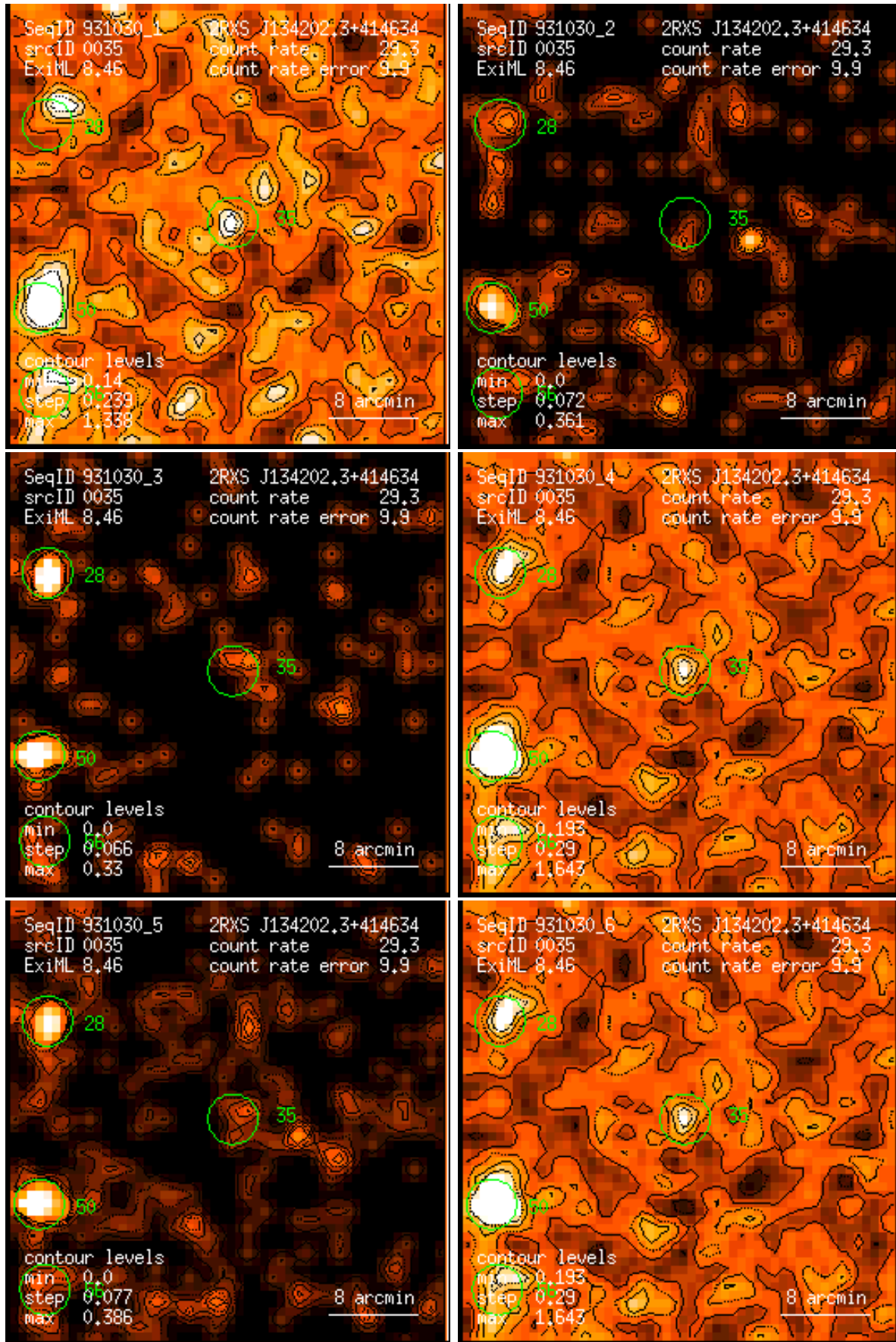
Figure 35: RASS 931030: detection 0035: band rate images, Gaussian filter: (1) PSPC channels 11 – 41, (2) 52 – 90, (3) 91 – 201, (4) 11 – 235, (5) 52 – 201, (6) 11 – 201. Broad band rates in counts/ks. Band rate contour levels in counts/ks/arcmin 2 .
