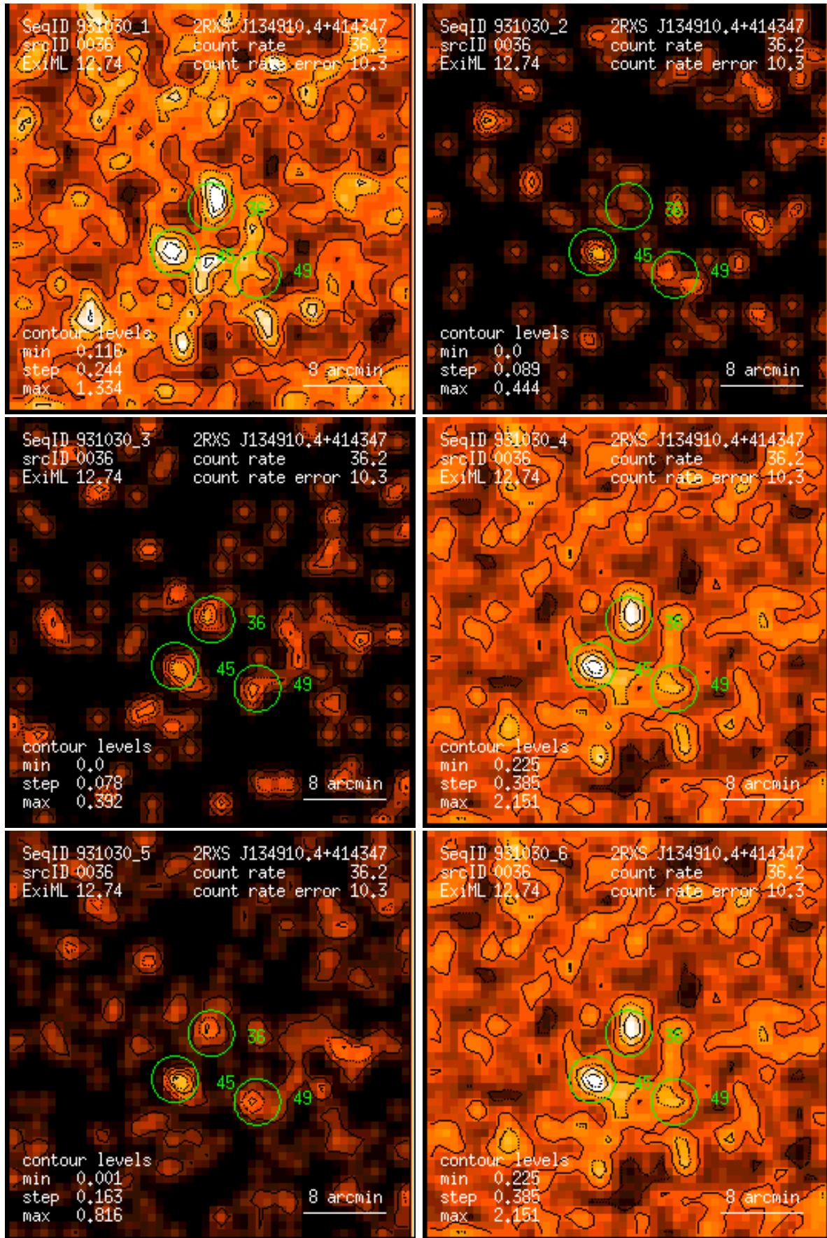
Figure 36: RASS 931030: detection 0036: band rate images, Gaussian filter: (1) PSPC channels 11 – 41, (2) 52 – 90, (3) 91 – 201, (4) 11 – 235, (5) 52 – 201, (6) 11 – 201. Broad band rates in counts/ks. Band rate contour levels in counts/ks/arcmin 2 .
